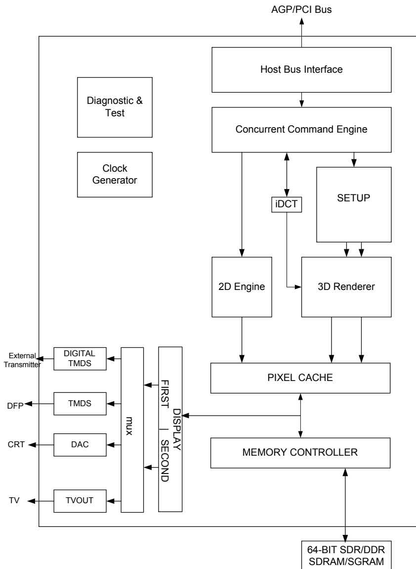
Figure 4-1. RV-100 Functional Block Diagram
