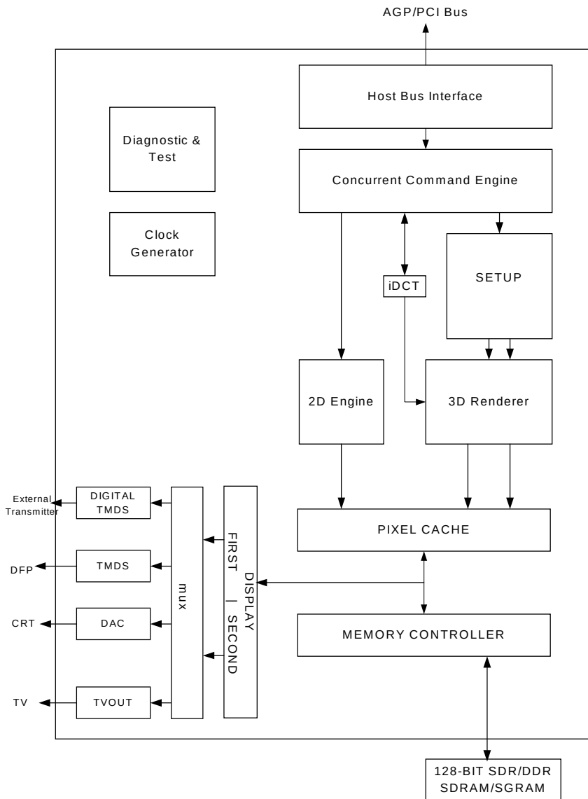
Figure 4-1. Radeon 7500 Functional Block Diagram
