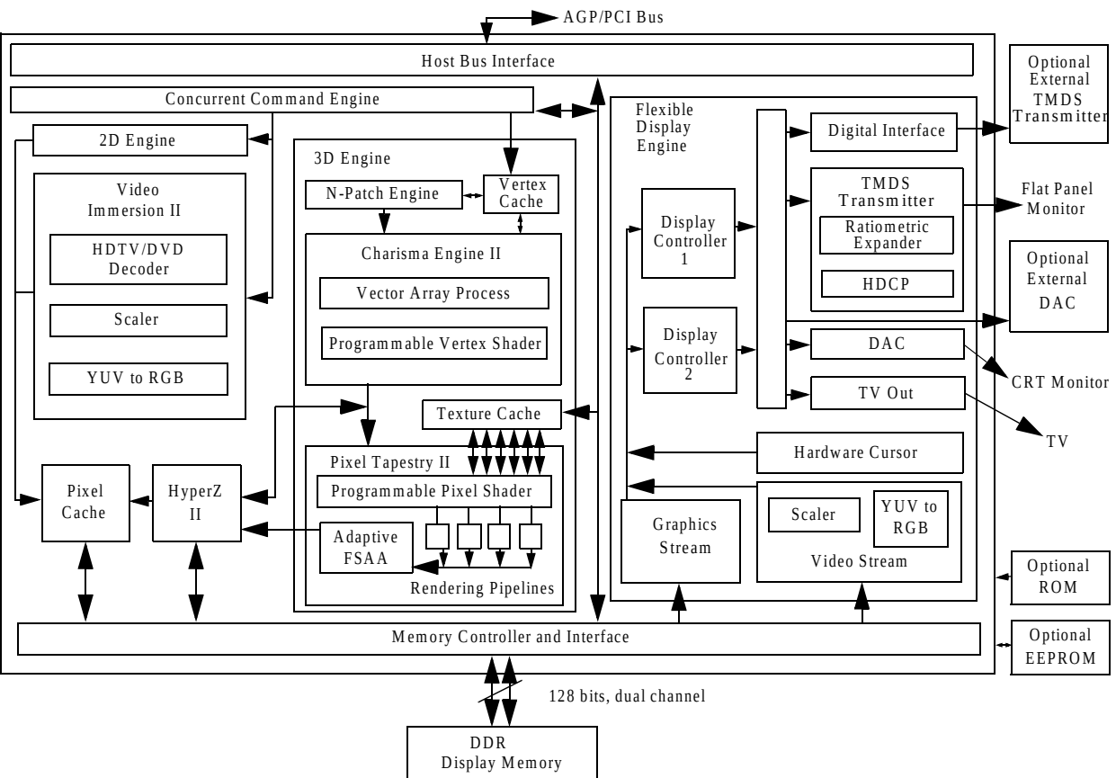
Figure 4-1. Radeon 8500 Functional Block Diagram
