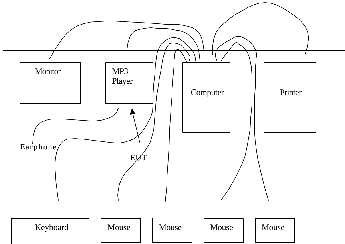
Figure 4-1 System layout
