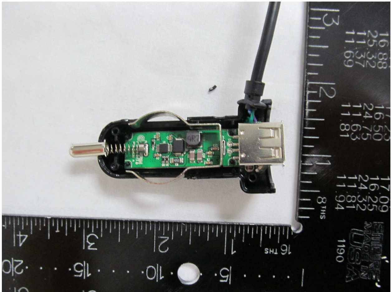
Cigaretted Lighter Enclosure
