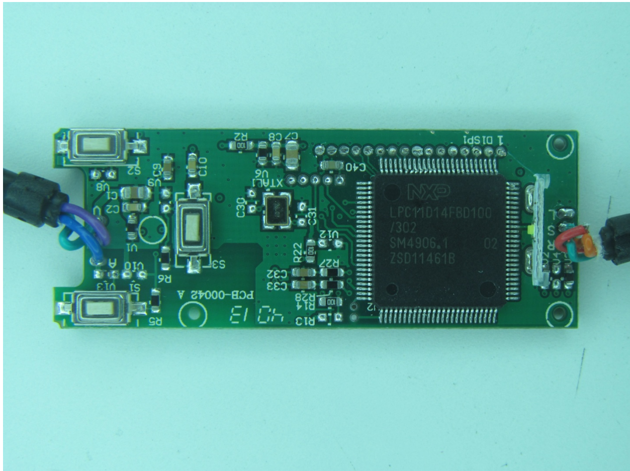
Transmitter Board with LCD Screen Removed
