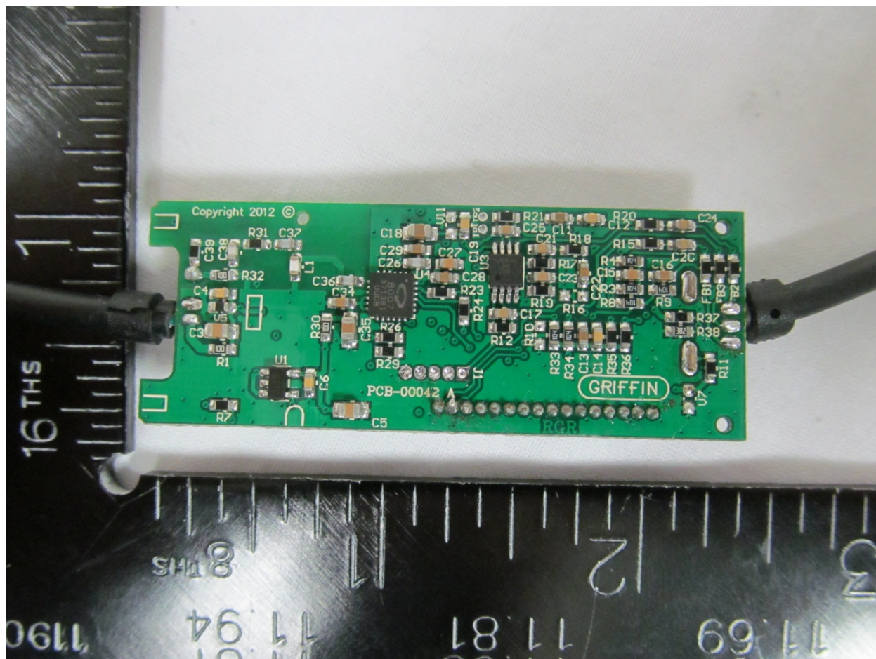
Transmitter Board
