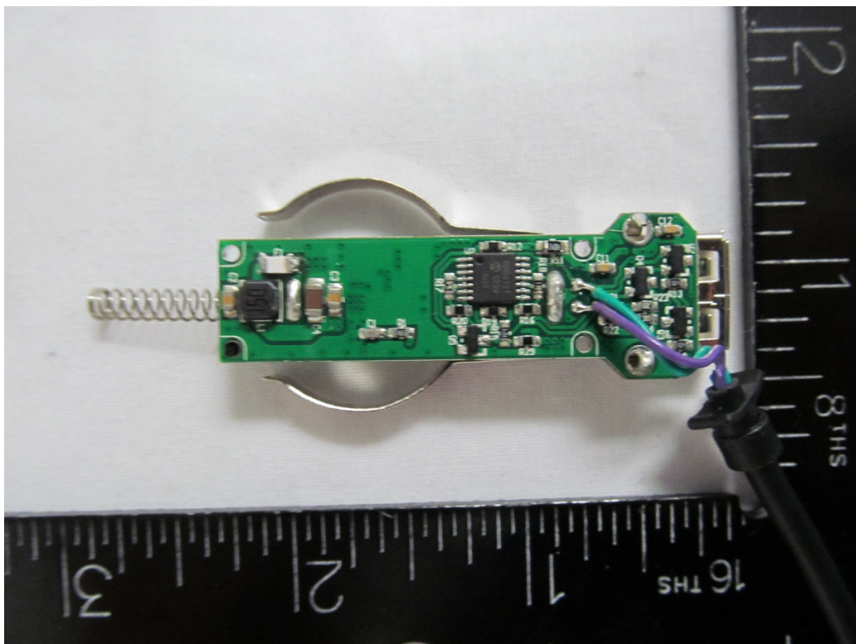
Cigaretted Lighter Board Detail
