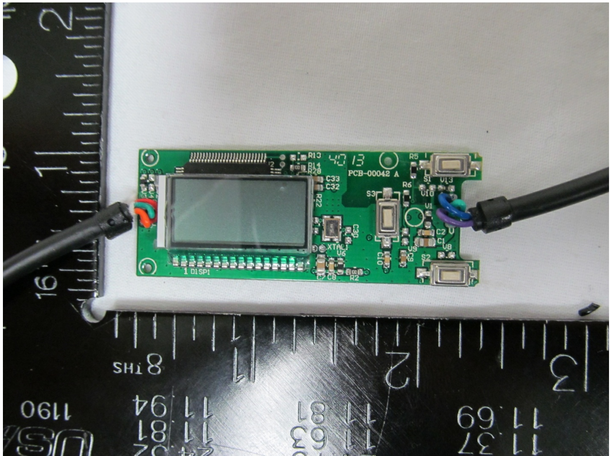
Transmitter Board
