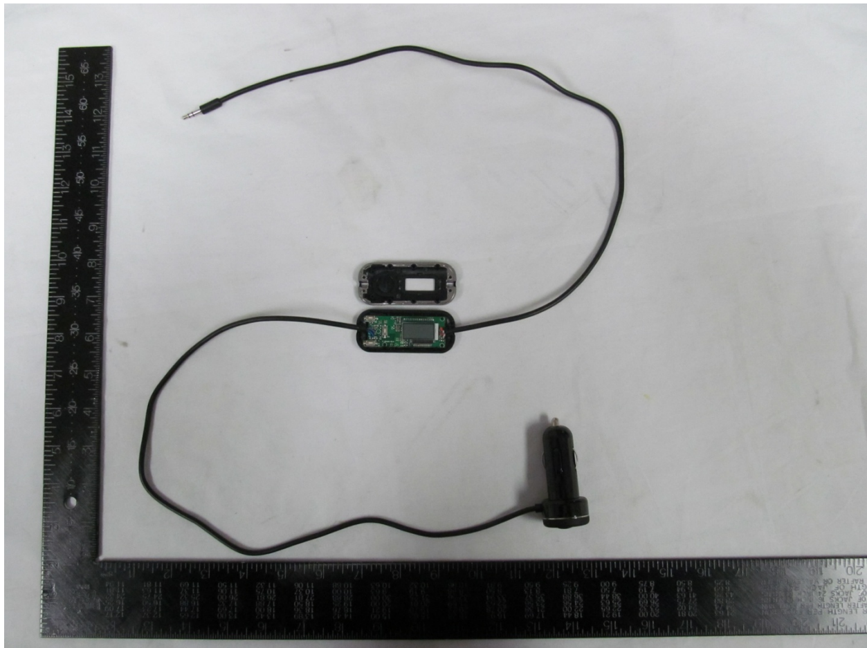
Transmitter Enclosure
