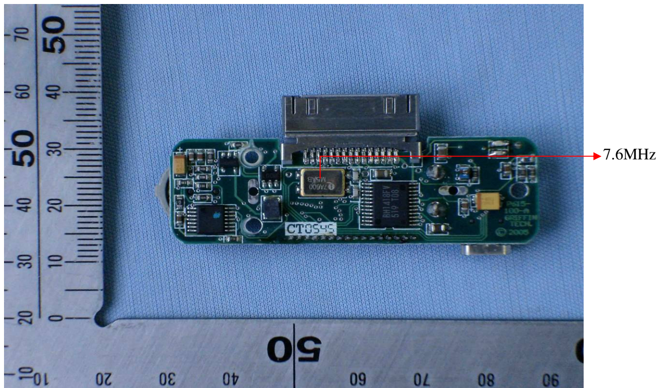
Full View of Component Side
