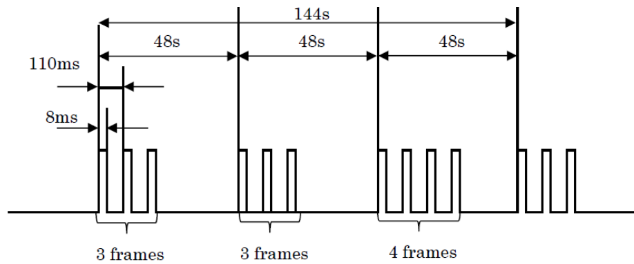
Plot 3: Timing of the transmitter (provided by manufacturer)
