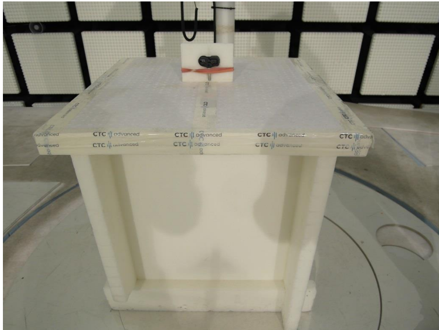
Photo 7: RSE set-up 9 kHz to 30 MHz
