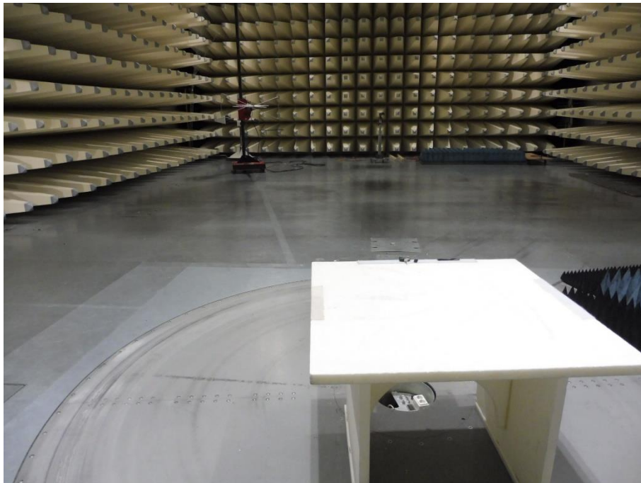
Photo 2: RSE set-up 30 MHz to 1 GHz
