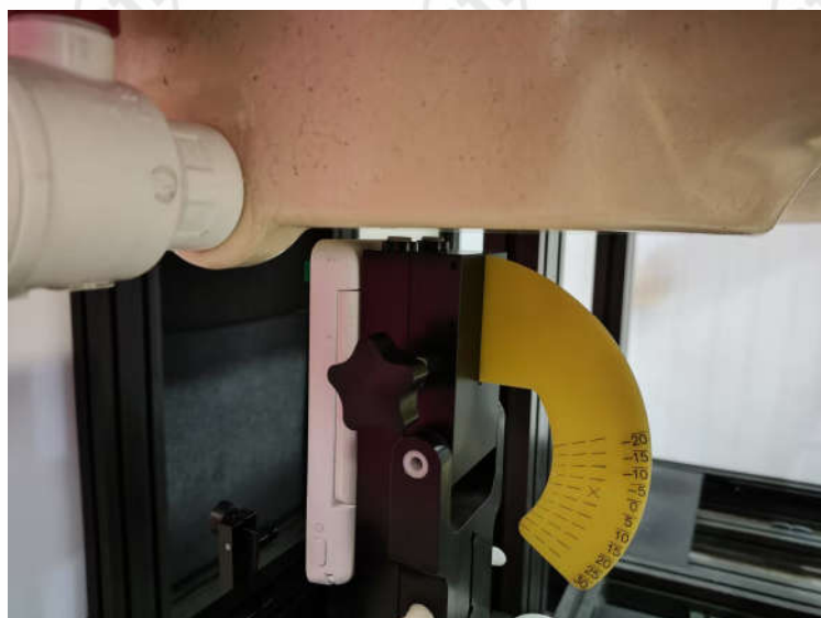
Photo 6: Left Side 5mm
