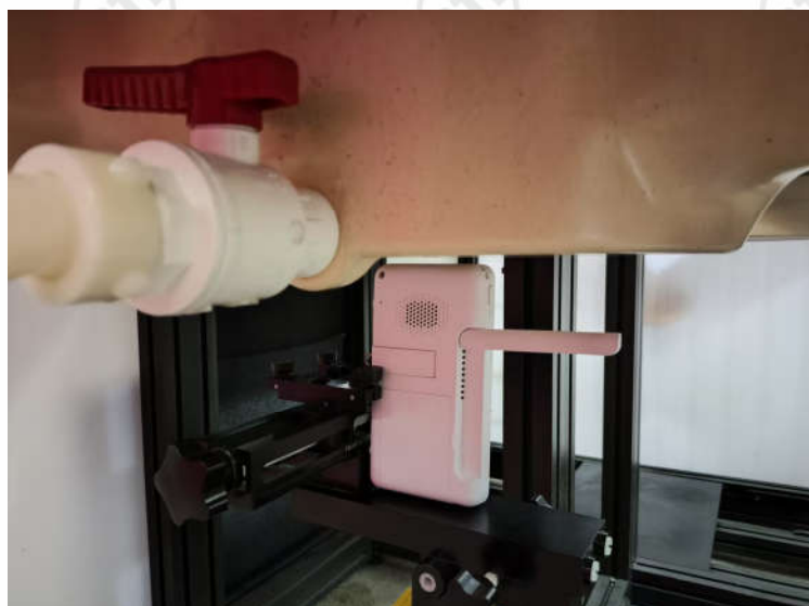
Photo 6: Right Side 5mm
