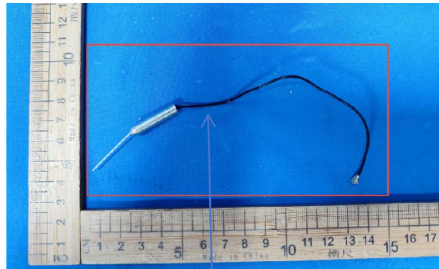
ANT Copper tube antenna
