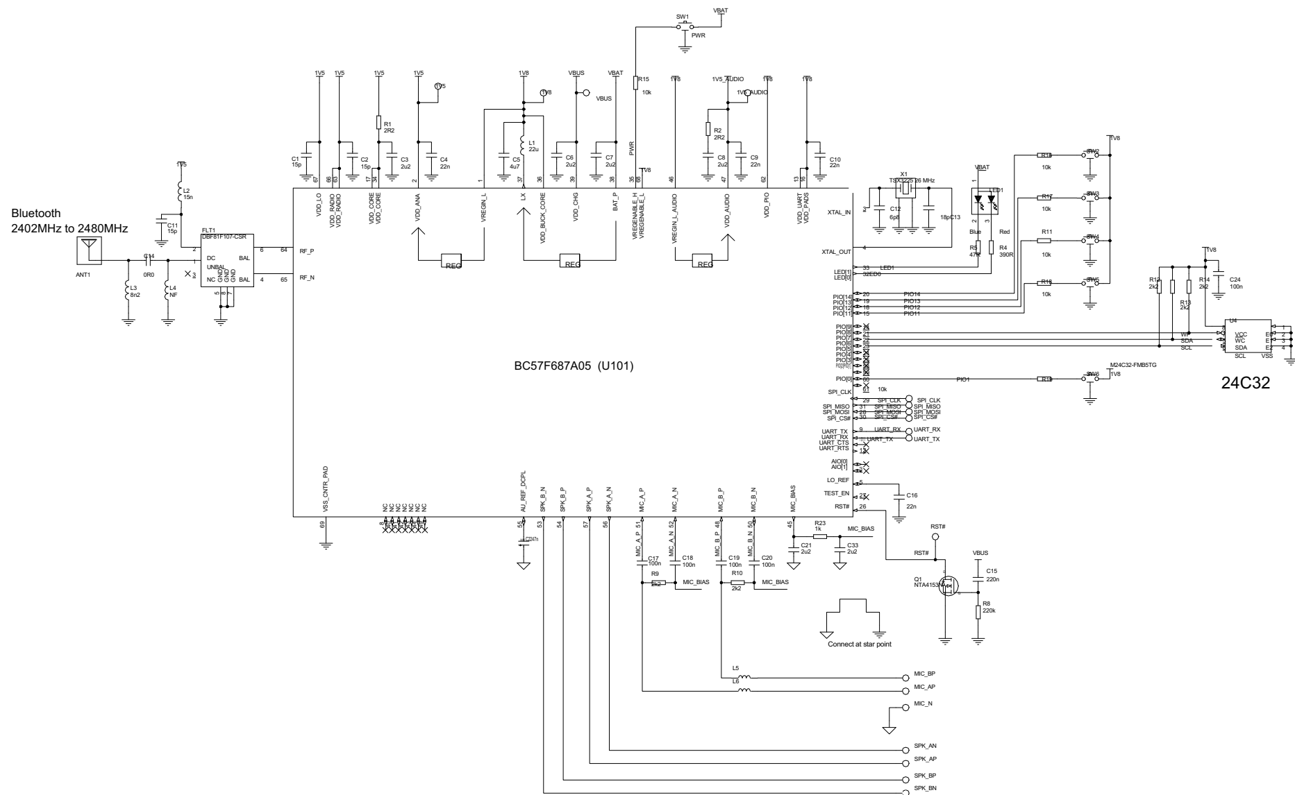
F-3088 Bluetooth module schematic
