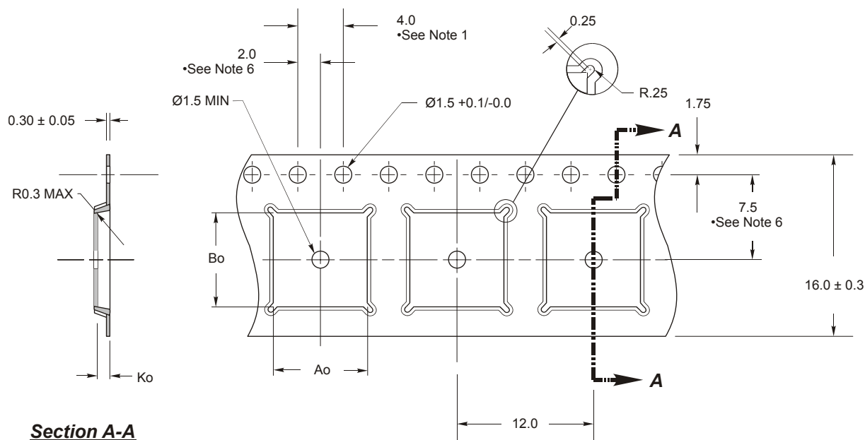
Figure 18.1: BlueTunes ROM QFN Tape Orientation
