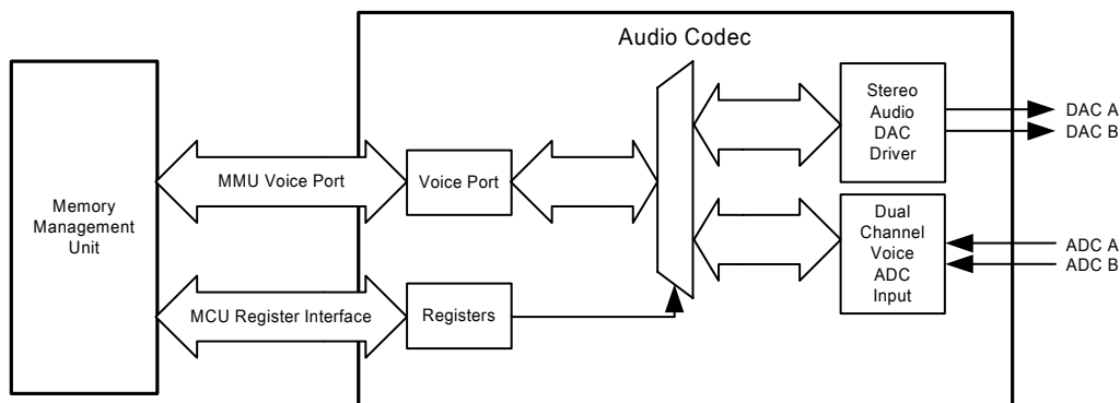
Figure 10.1: BlueTunes ROM QFN Audio Interface
