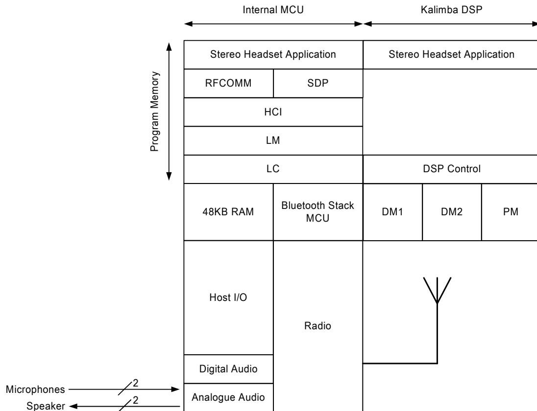
Figure 16.1: Stand-alone Application: BlueTunes ROM Stereo Headset Solution
