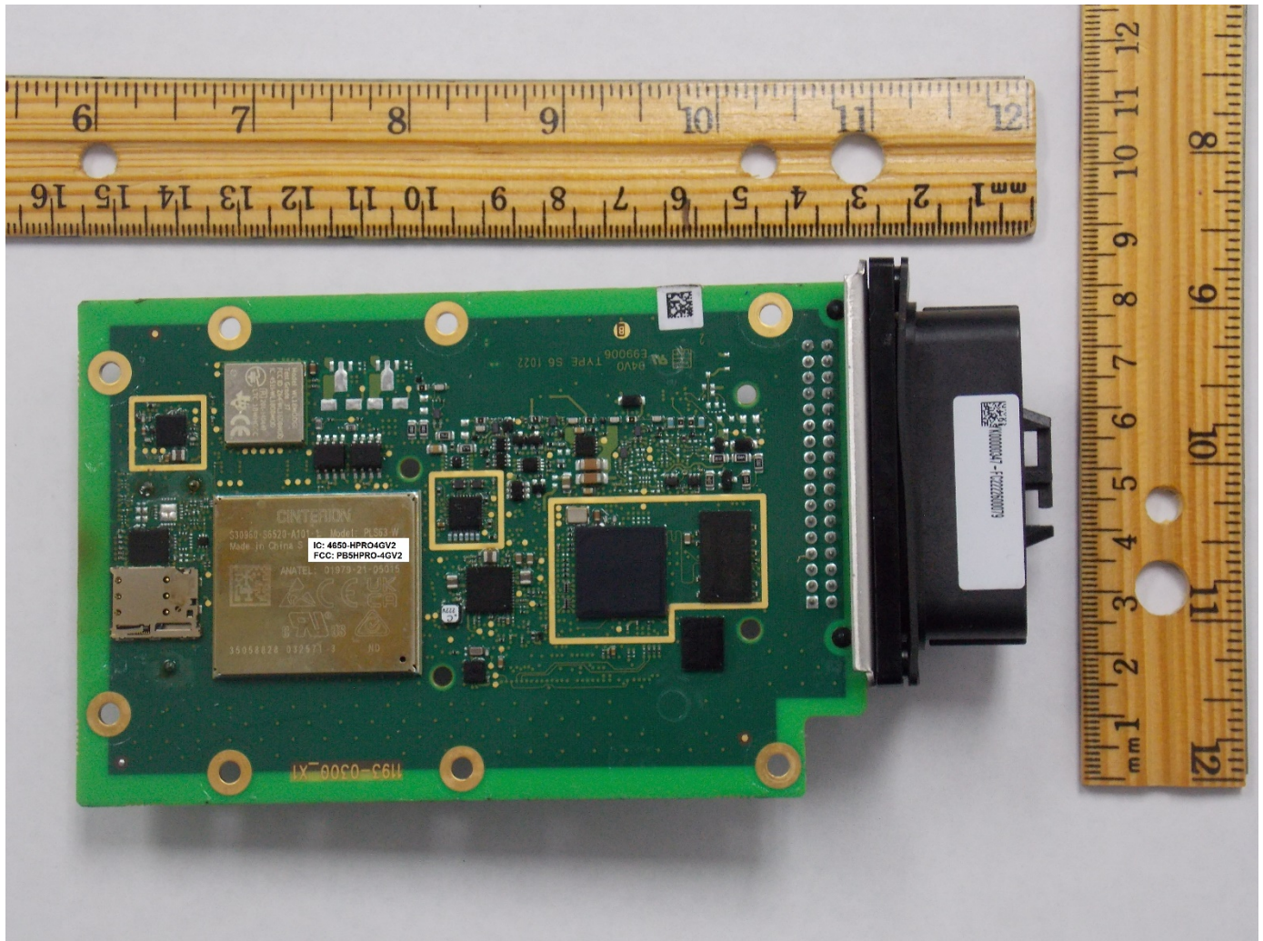
Back Side of PCB
