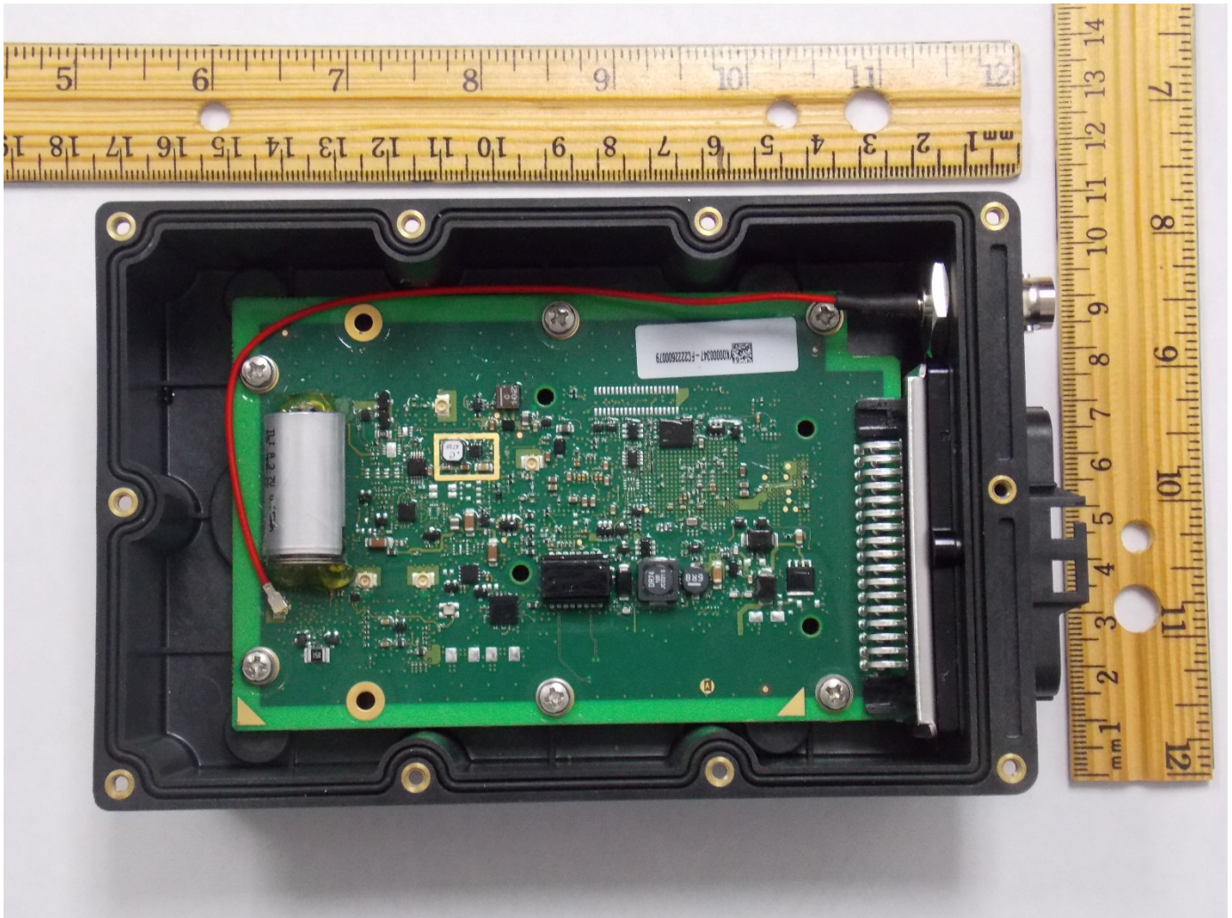
Top Cover Removed
