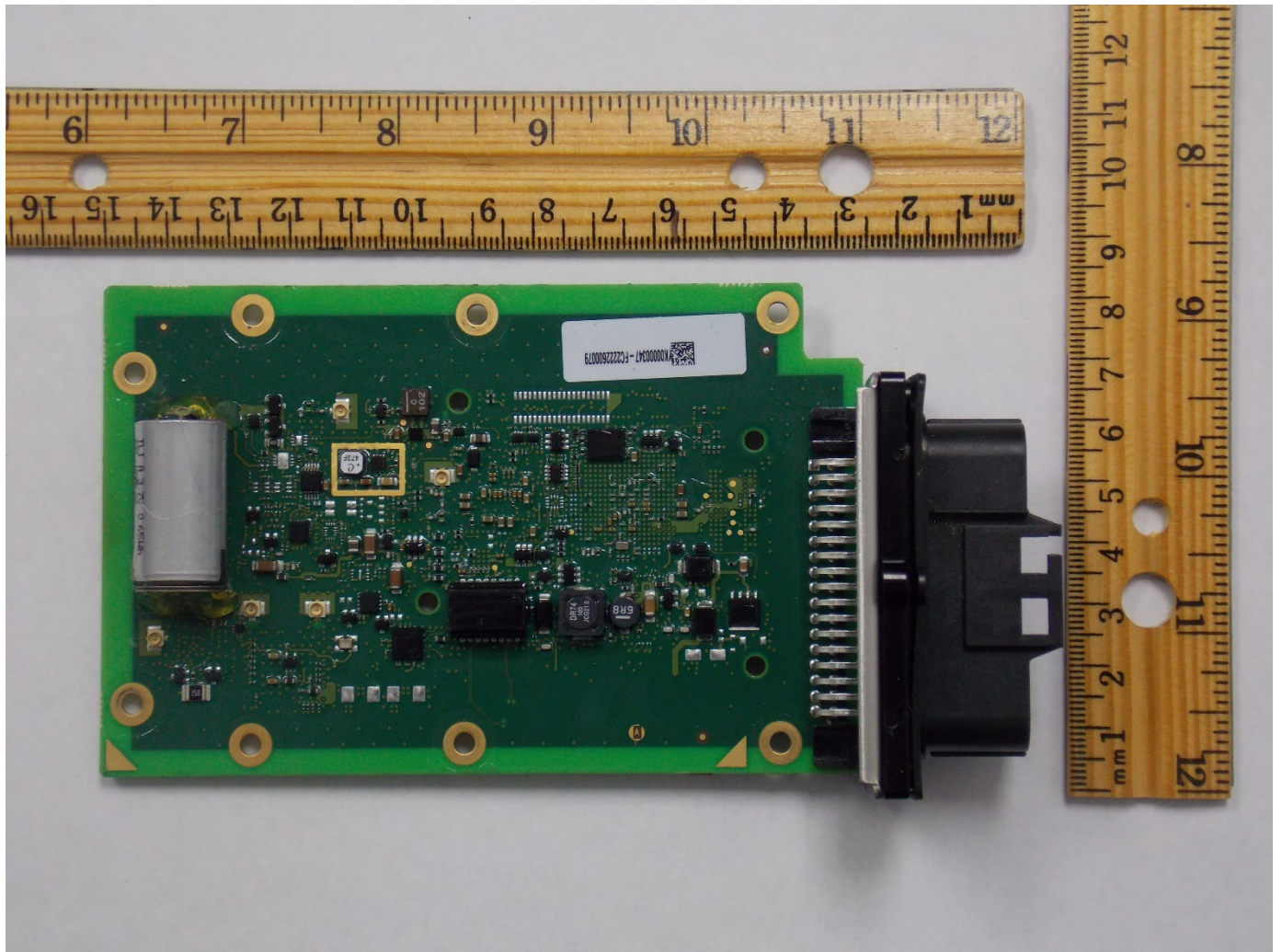
Top Side of PCB
