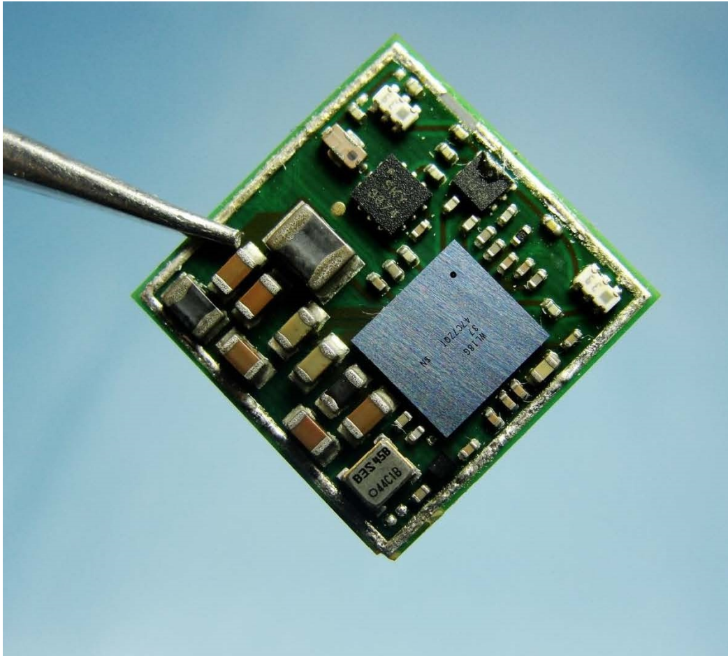
WiFi Module Front View with the Shield Removed Close Up
