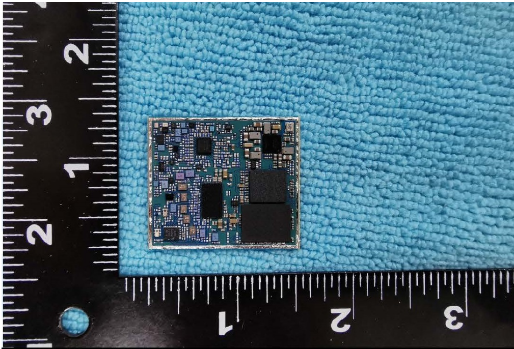
Cellular Module Front View with the Shield Cover Removed
