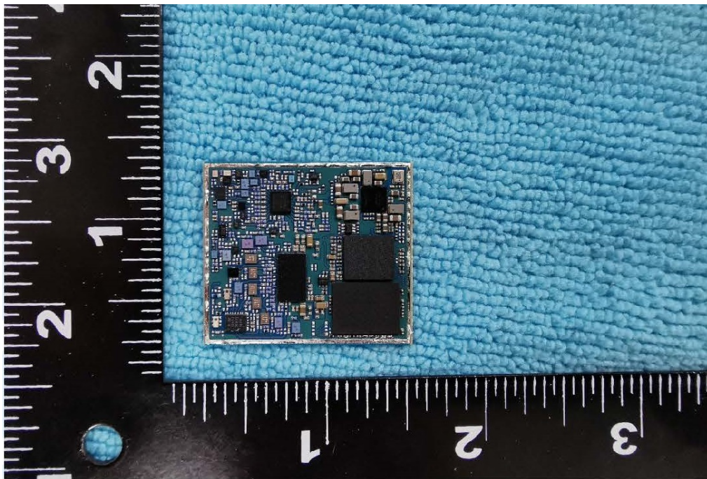
Cellular Module Back View
