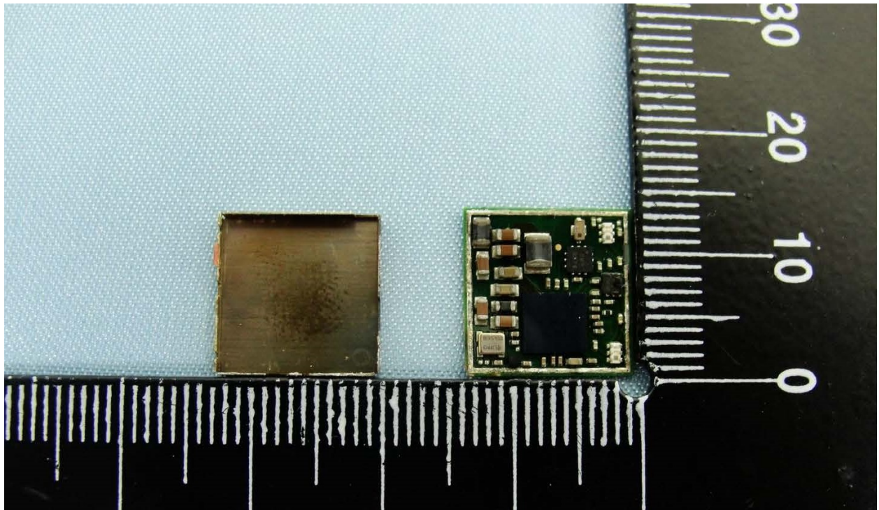
WiFi Module Front View with the Shield Cover Removed
