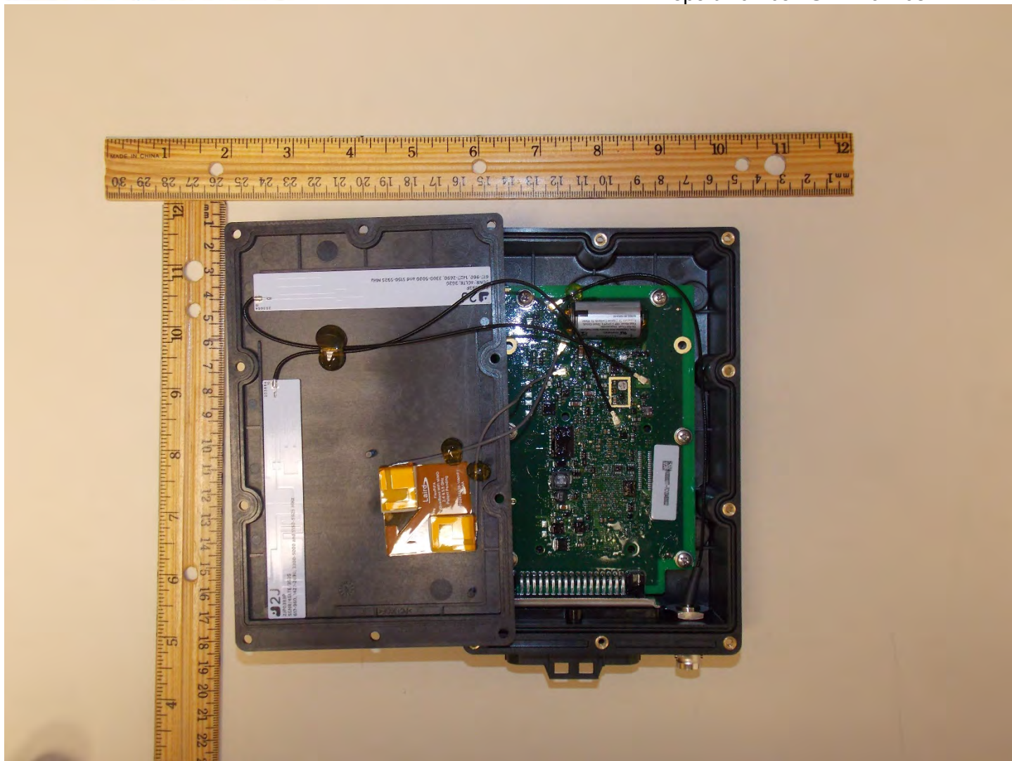
Cover Open Showing Antennas
