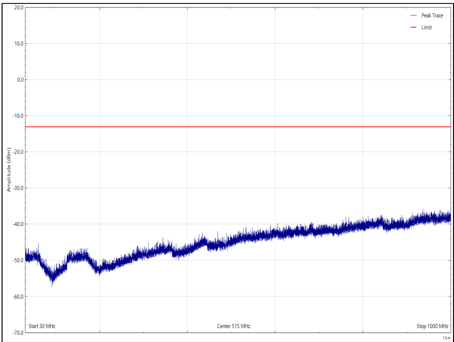
Figure 43 - 1621.020833 MHz, 30 MHz to 1 GHz Polarisation: Vertical, EUT Orientation: Y
