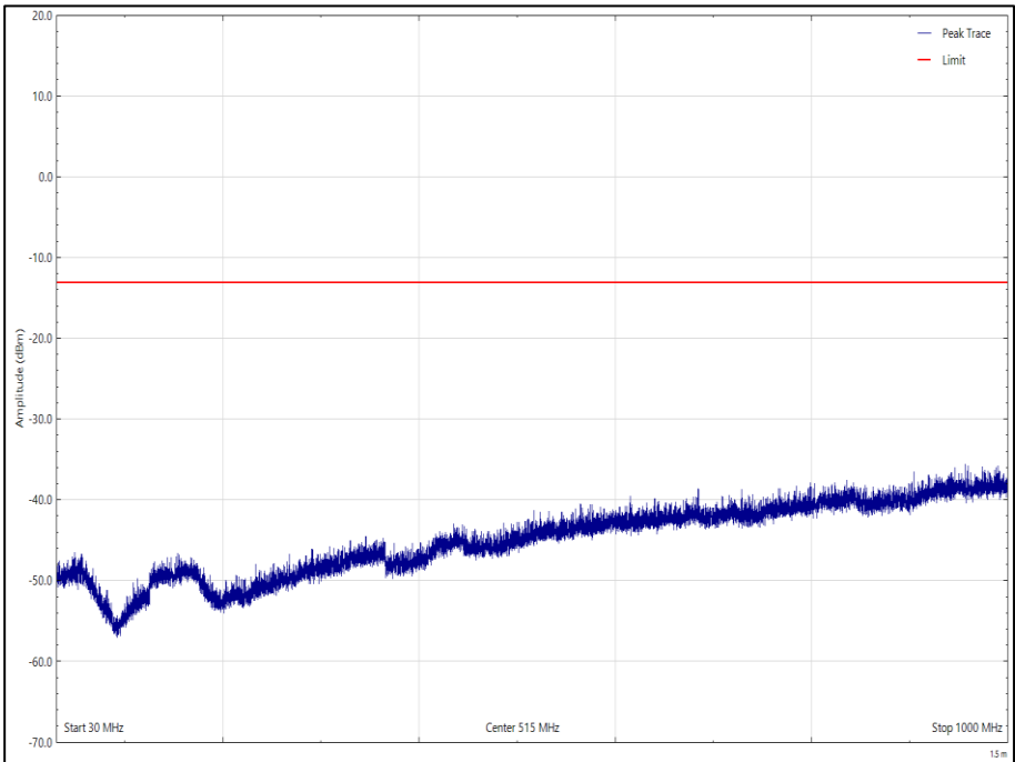
Figure 30 - 1616.020833 MHz, 30 MHz to 1 GHz Polarisation: Horizontal, EUT Orientation: Y
