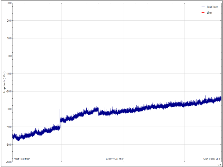
Figure 48 - 1621.020833 MHz - 1 GHz to 18 GHz Polarisation: Horizontal, EUT Orientation: Y
