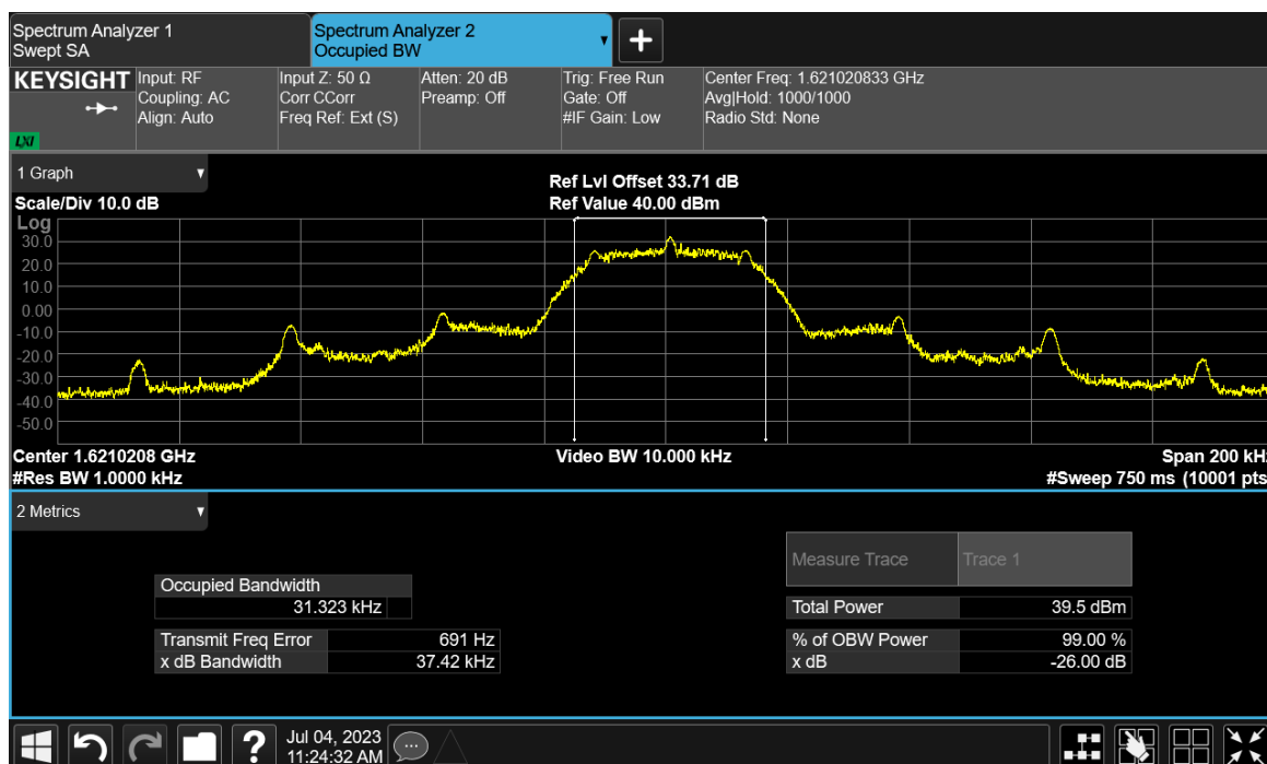
Figure 5 - 1621.020833 MHz
