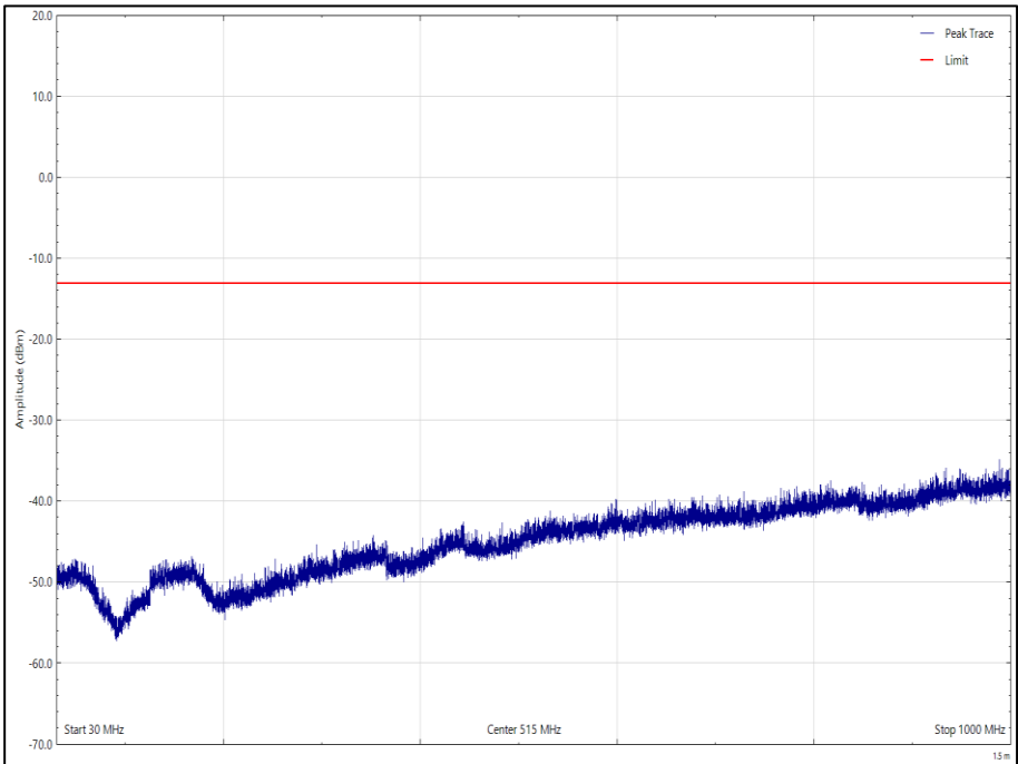
Figure 32 - 1616.020833 MHz, 30 MHz to 1 GHz Polarisation: Horizontal, EUT Orientation: Z
