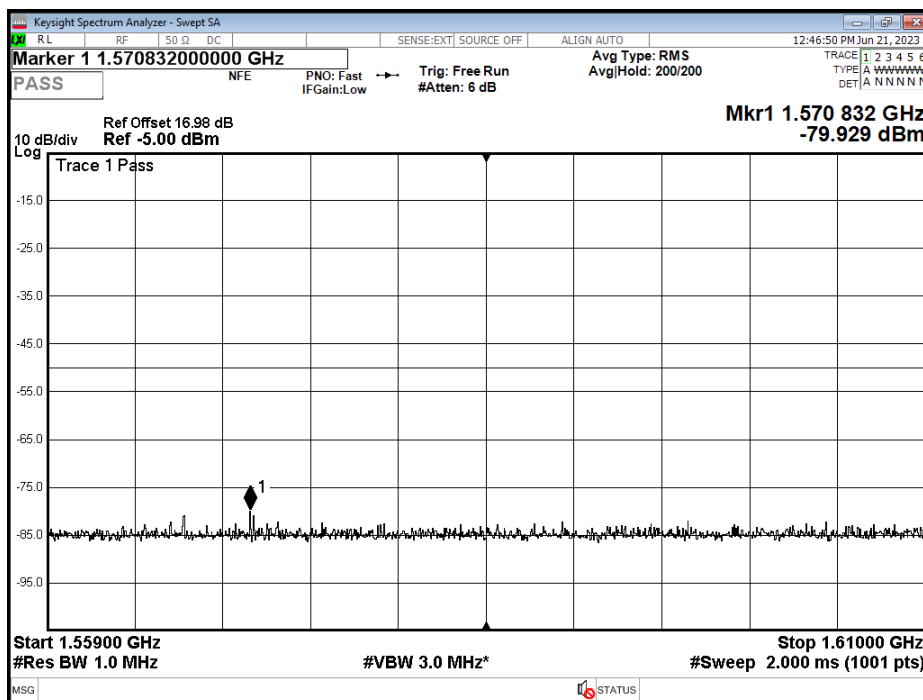
Figure 70 - Carrier-off state
