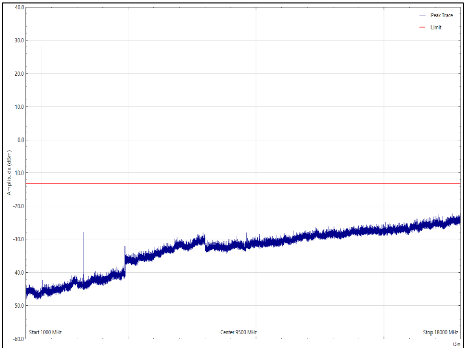
Figure 63 - 1625.979167 MHz - 1 GHz to 18 GHz Polarisation: Vertical, EUT Orientation: Z
