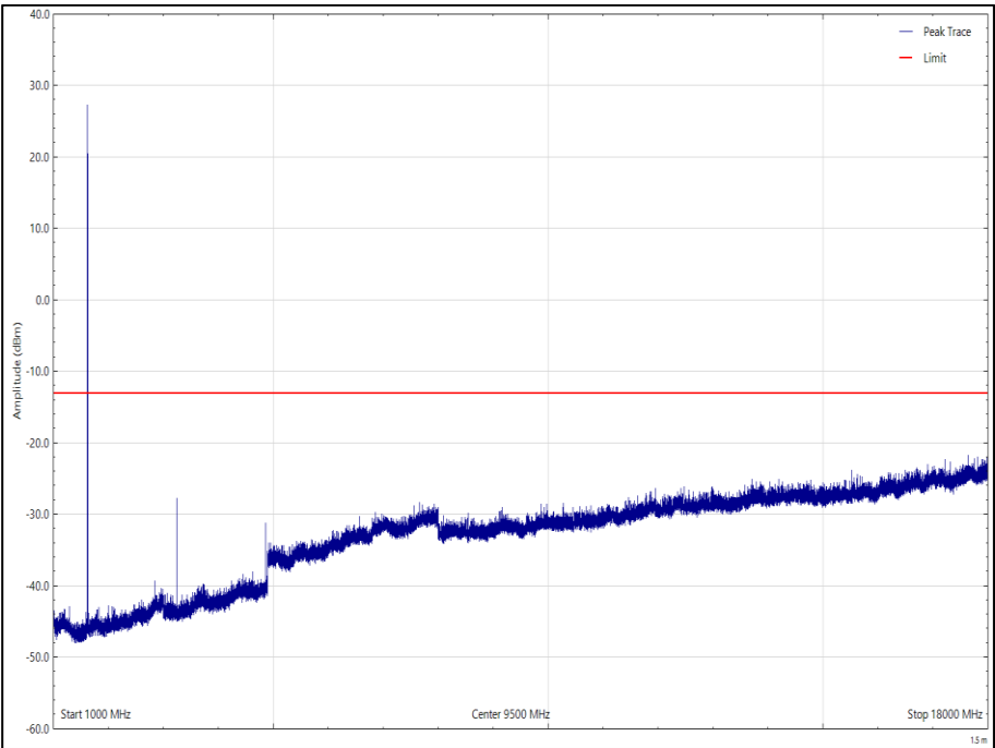
Figure 47 - 1621.020833 MHz - 1 GHz to 18 GHz Polarisation: Vertical, EUT Orientation: X
