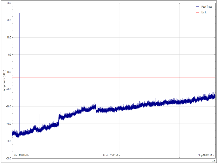
Figure 62 - 1625.979167 MHz - 1 GHz to 18 GHz Polarisation: Horizontal, EUT Orientation: Z
