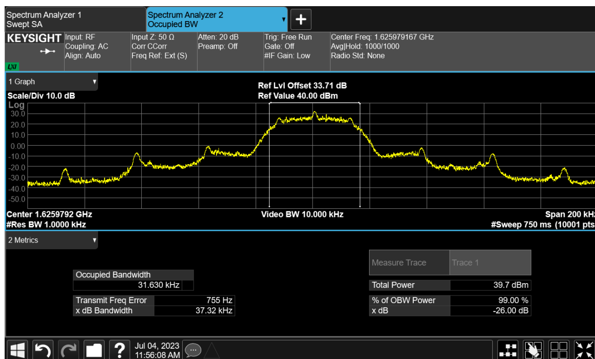
Figure 6 - 1625.979167 MHz
