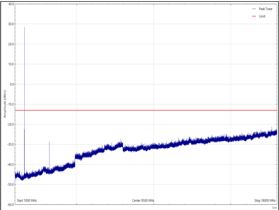
Figure 35 - 1616.020833 MHz - 1 GHz to 18 GHz Polarisation: Vertical, EUT Orientation: X
