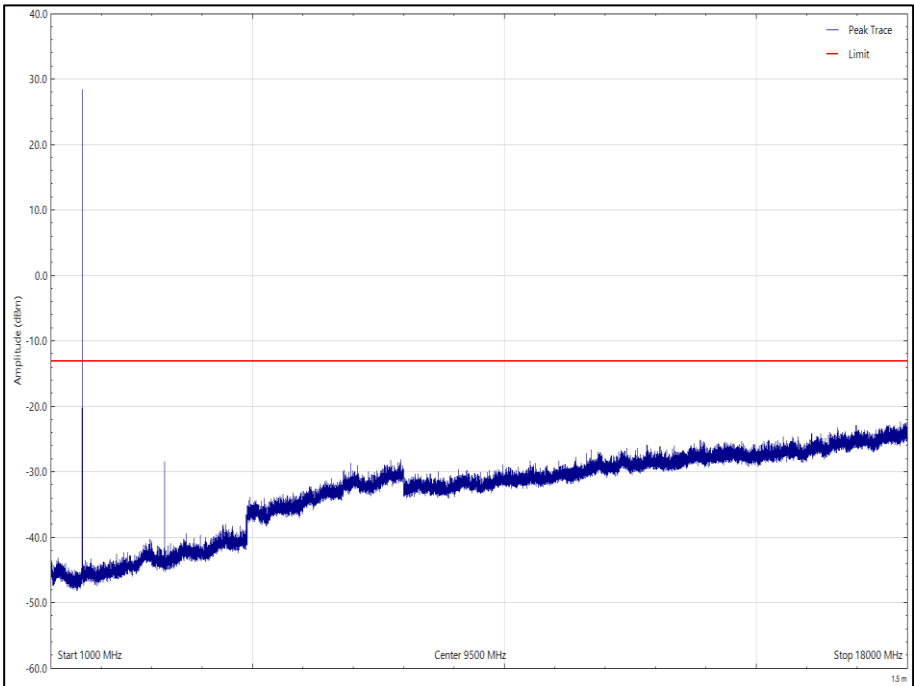
Figure 61 - 1625.979167 MHz - 1 GHz to 18 GHz Polarisation: Vertical, EUT Orientation: Y
