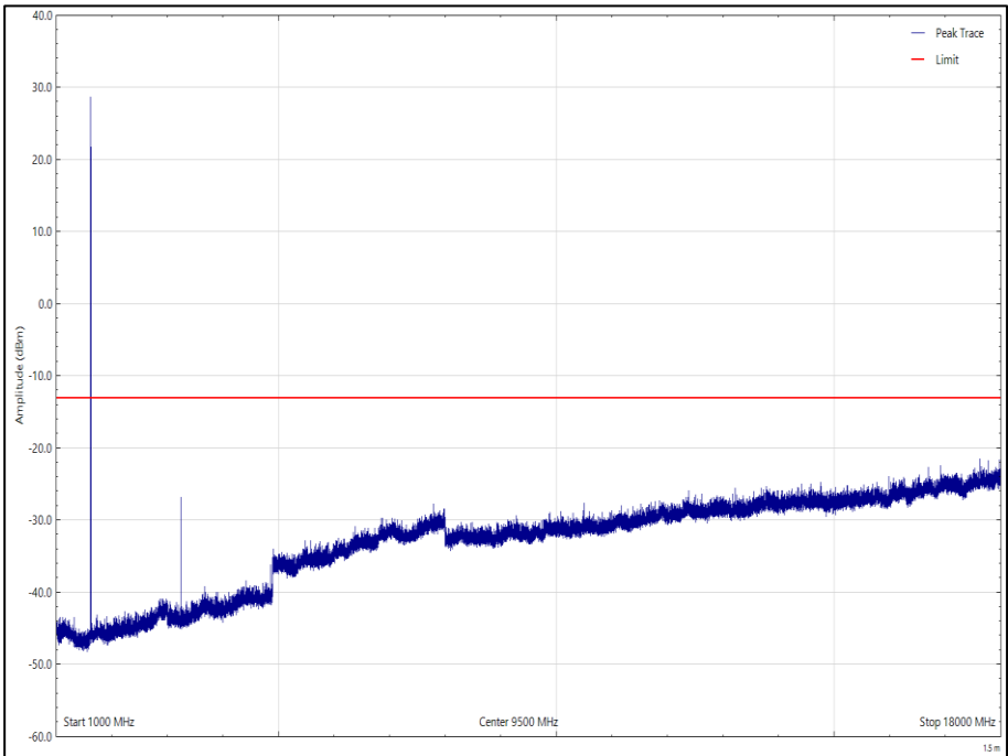
Figure 51 - 1621.020833 MHz - 1 GHz to 18 GHz Polarisation: Vertical, EUT Orientation: Z
