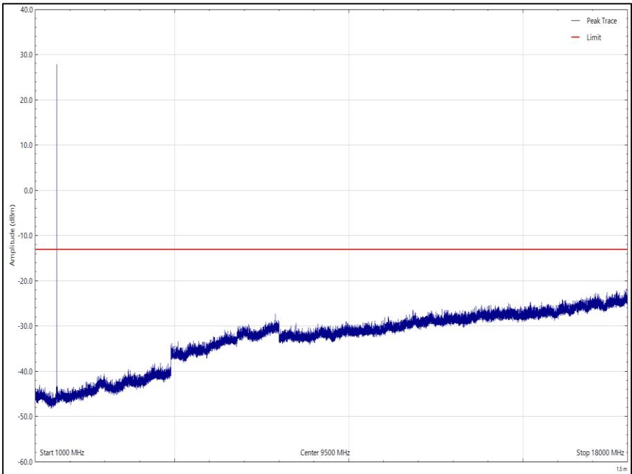
Figure 39 - 1616.020833 MHz - 1 GHz to 18 GHz Polarisation: Vertical, EUT Orientation: Z
