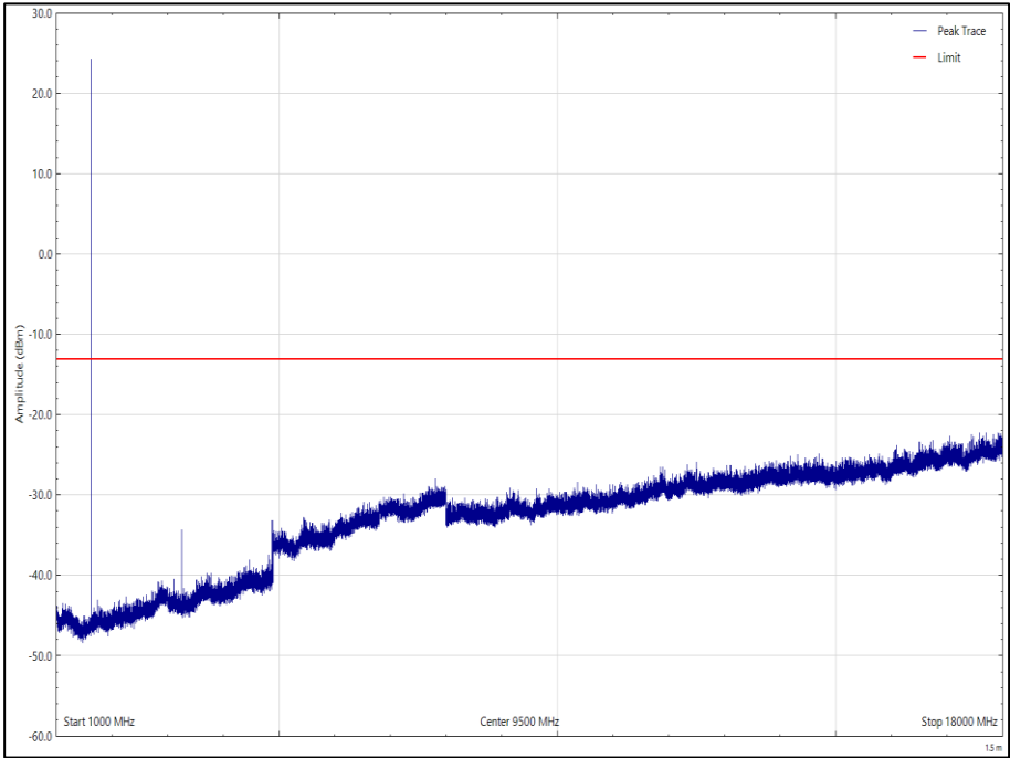
Figure 60 - 1625.979167 MHz - 1 GHz to 18 GHz Polarisation: Horizontal, EUT Orientation: Y
