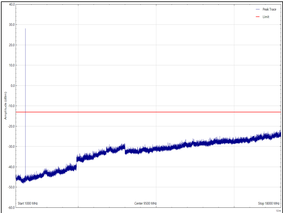
Figure 37 - 1616.020833 MHz - 1 GHz to 18 GHz Polarisation: Vertical, EUT Orientation: Y
