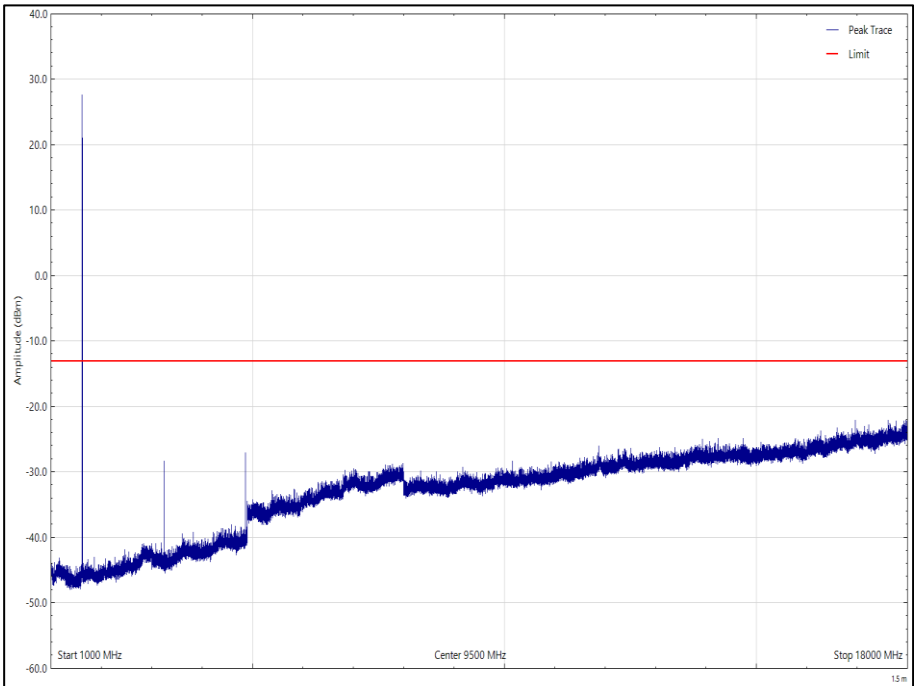
Figure 49 - 1621.020833 MHz - 1 GHz to 18 GHz Polarisation: Vertical, EUT Orientation: Y
