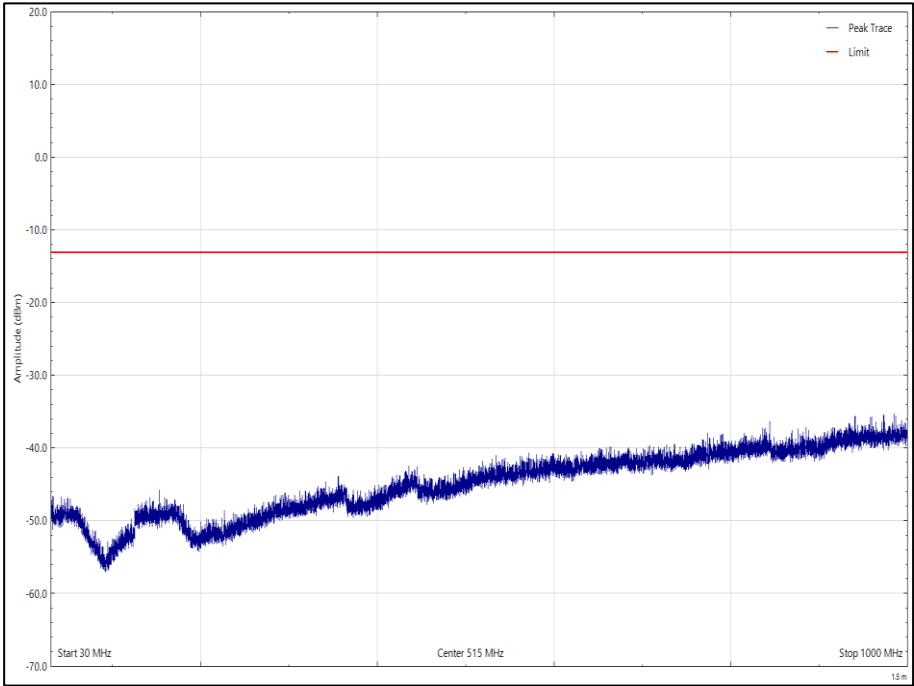
Figure 44 - 1621.020833 MHz, 30 MHz to 1 GHz Polarisation: Horizontal, EUT Orientation: Z
