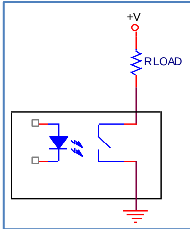
Figure 5-4: SW_GND
