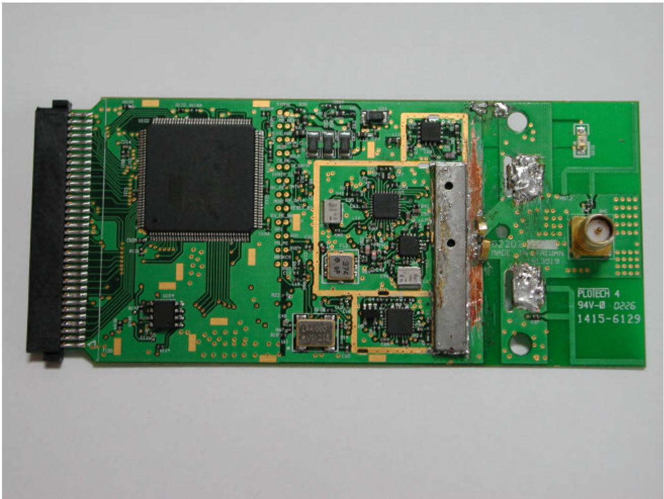
Internal Photo of the TeLLUS C100
