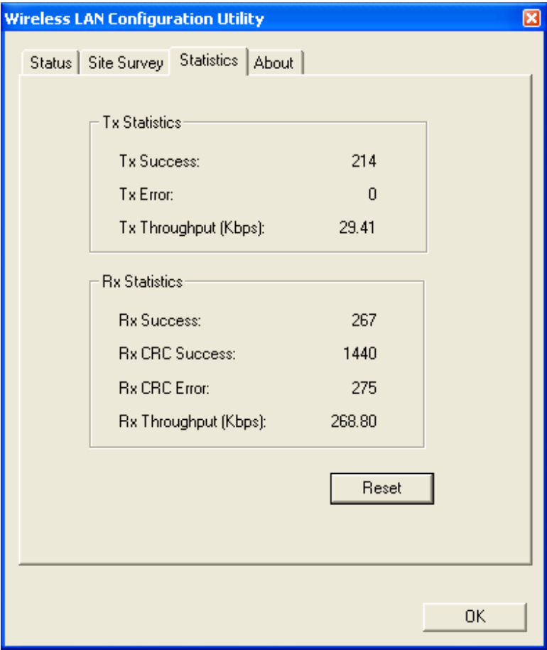
Figure 3-8 Statistics page
