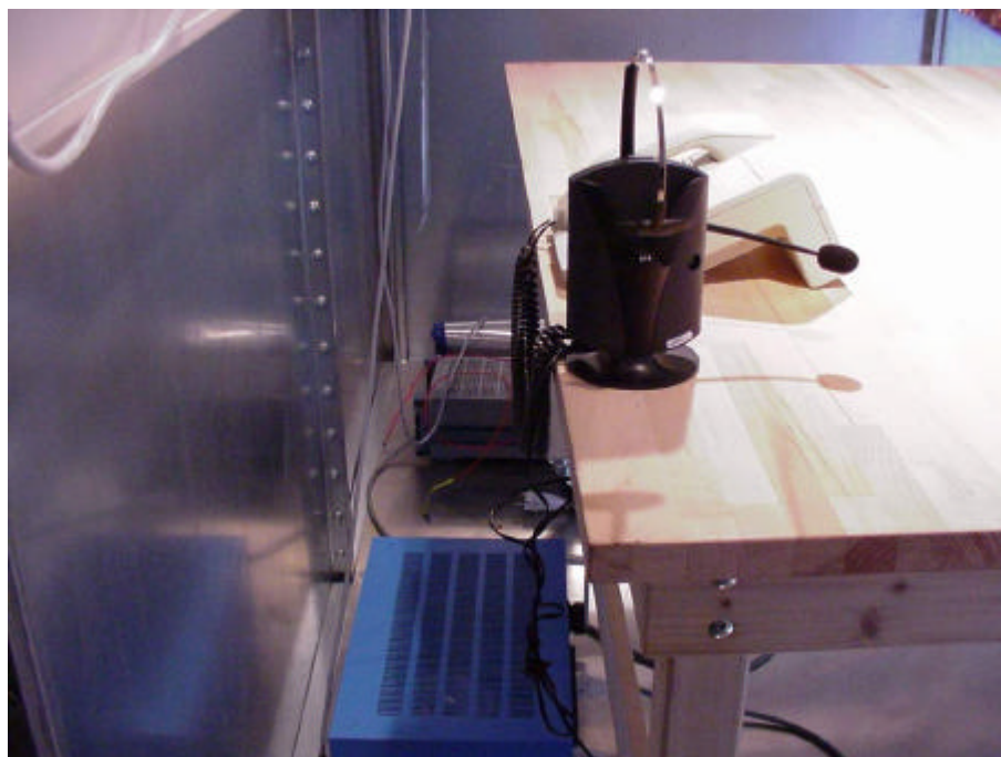
Picture 2 : Setup for AC mains measurements rear view)
