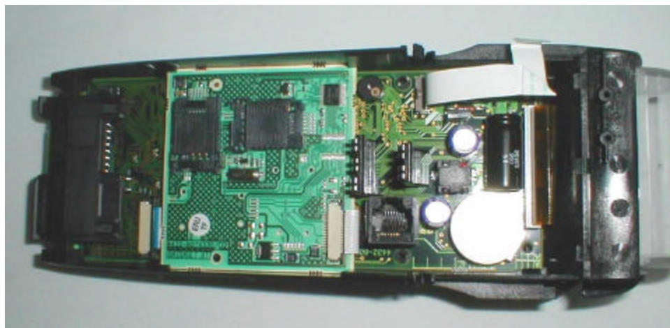
Bottom with RF Module Removed
