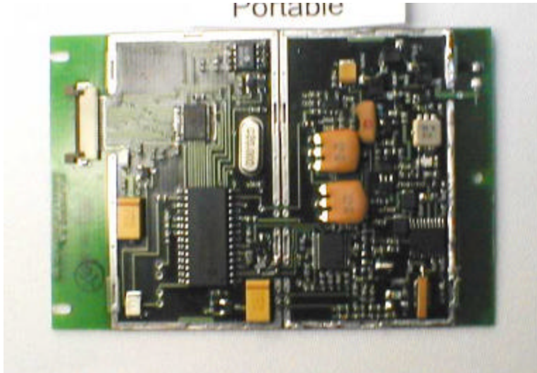
RF Module PCB Shield Removed
