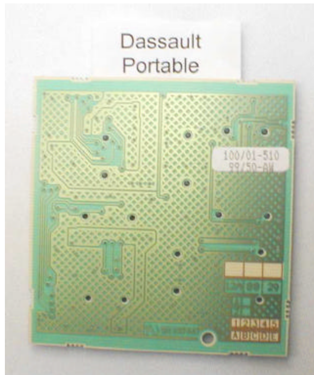
Lower PCB Bottom
