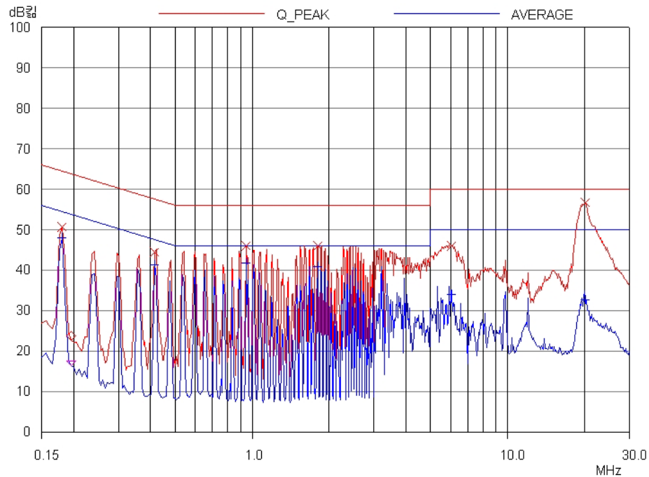
HOT LINE
