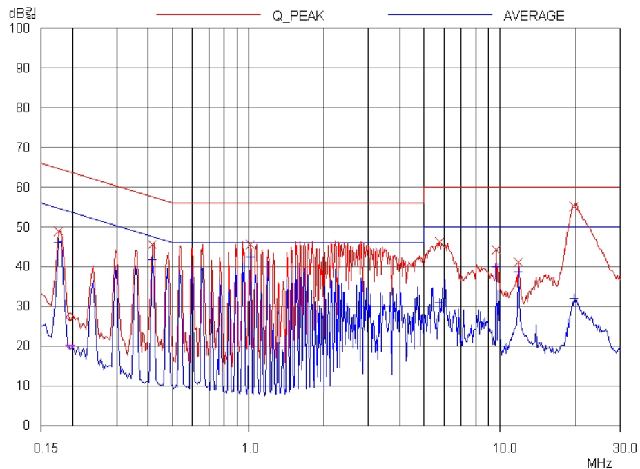
NEUTRAL LINE
