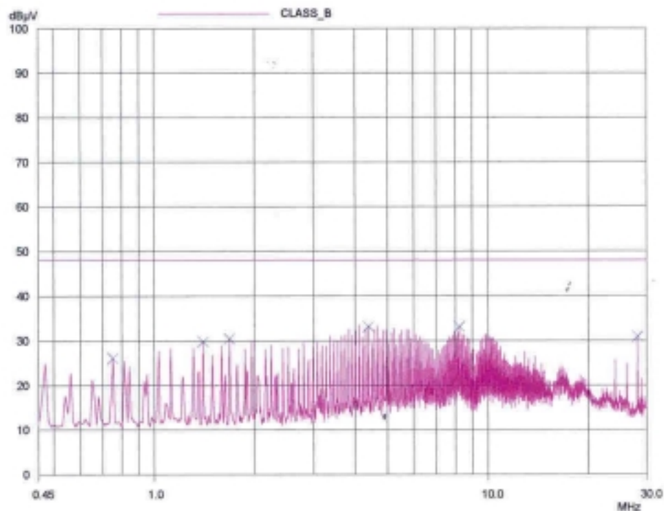
HOT LINE
