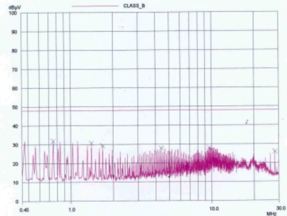
NEUTRAL LINE
