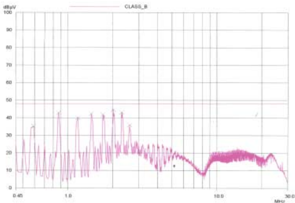
NEUTRAL LINE
