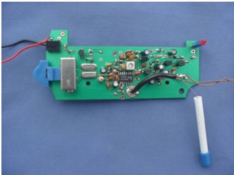
Figure 4. General Appearance of the PCB, Front View
