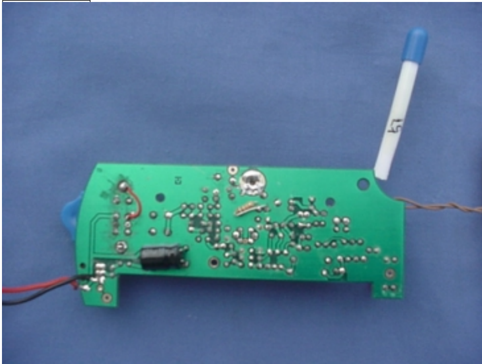
Figure 5. General Appearance of the PCB, Rear View
