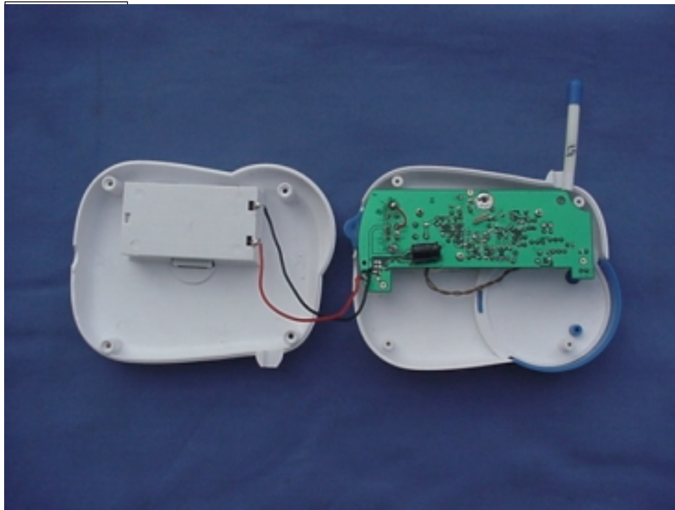
Figure 3. Cover Opened
