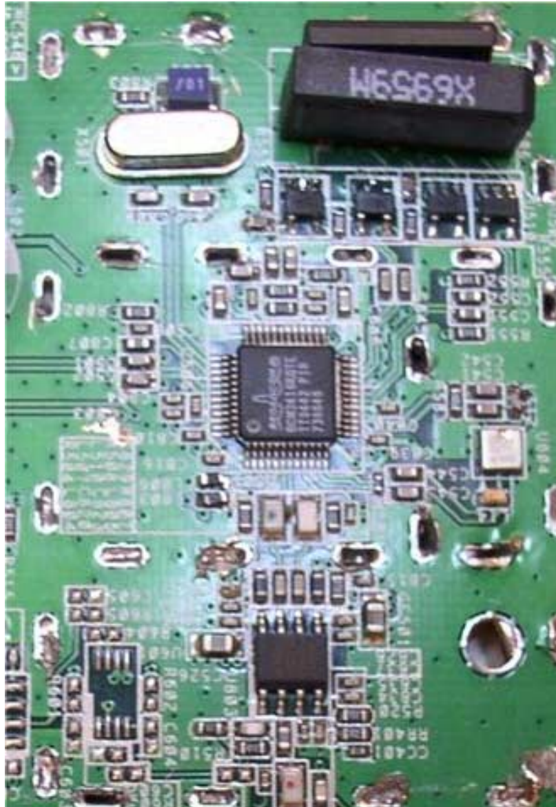
Photograph No.4 RF part with shields removed
