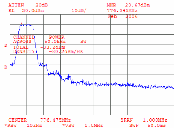
Plot 7.4.8 Adjacent channel coupled power measurements, low carrier frequency, QPSK
