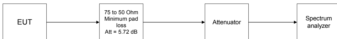
Figure 7.8.1 Occupied bandwidth test setup
