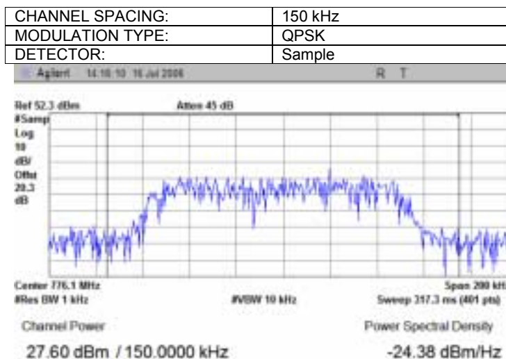
Plot 7.1.1 Average output power test results at low frequency
