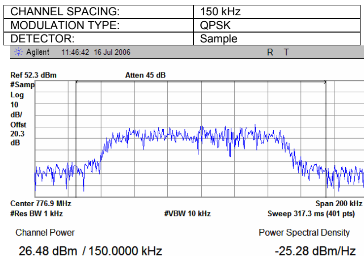
Plot 7.1.5 Average output power test results at high frequency
