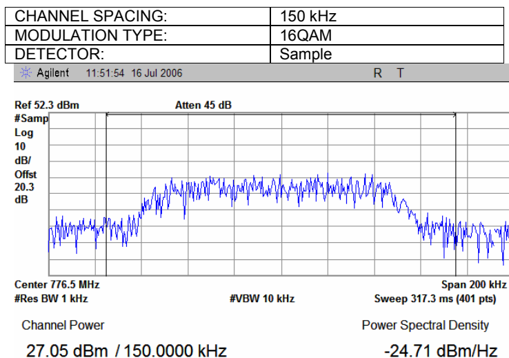
Plot 7.1.9 Average output power test results at mid frequency
