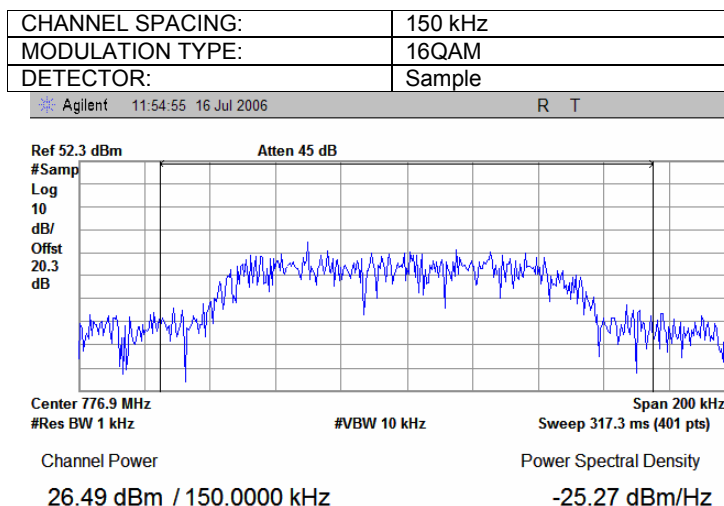
Plot 7.1.11 Average output power test results at high frequency
