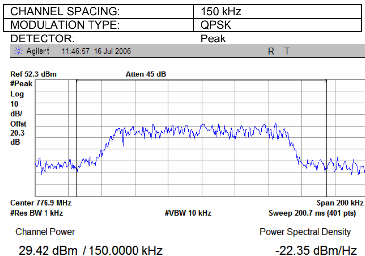
Plot 7.1.6 Peak output power test results at high frequency
