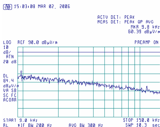
Plot 7.5.6 Radiated emission measurements in 9 - 150 kHz range
