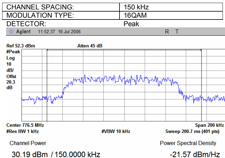
Plot 7.1.10 Peak output power test results at mid frequency
