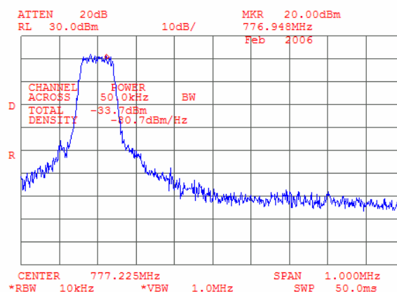
Plot 7.4.65 Adjacent channel coupled power measurements, high carrier frequency, 16QAM
