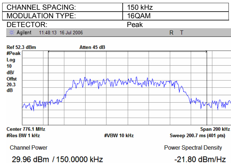
Plot 7.1.8 Peak output power test results at low frequency
