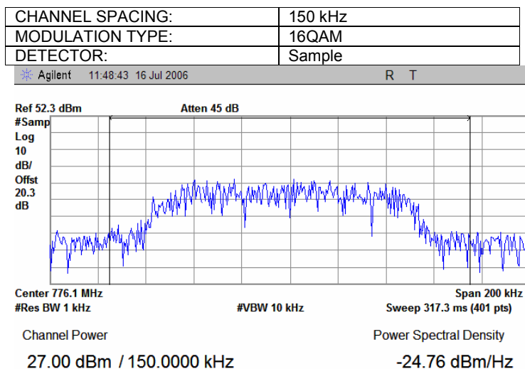
Plot 7.1.7 Average output power test results at low frequency
