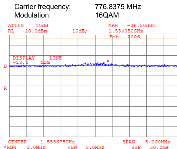
Plot 7.3.15 Spurious emission measurements at RF antenna connector, the 2 nd harmonic of the high channel
