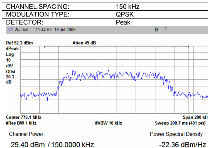
Plot 7.1.2 Peak output power test results at low frequency
