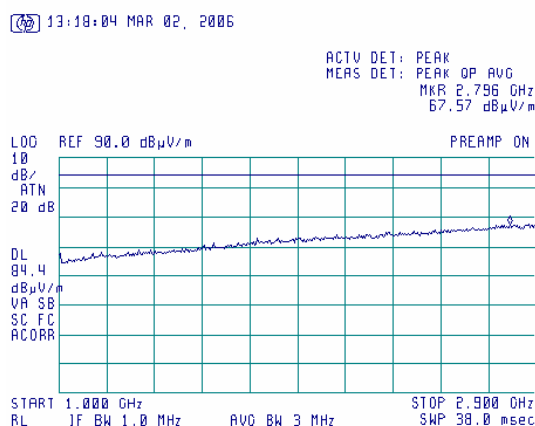
Plot 7.5.22 Radiated emission measurements in 1 – 2.9 GHz range
