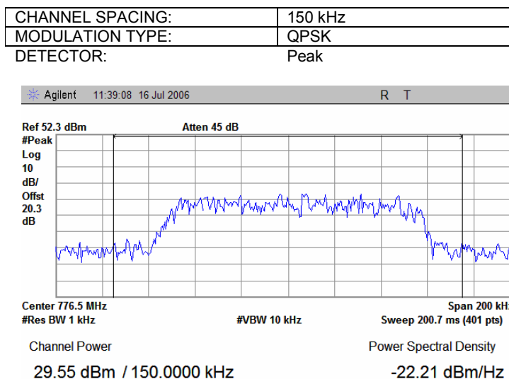
Plot 7.1.4 Peak output power test results at mid frequency
