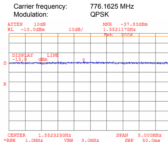
Plot 7.3.31 Spurious emission measurements at RF antenna connector, the 2 nd harmonic of the low channel
