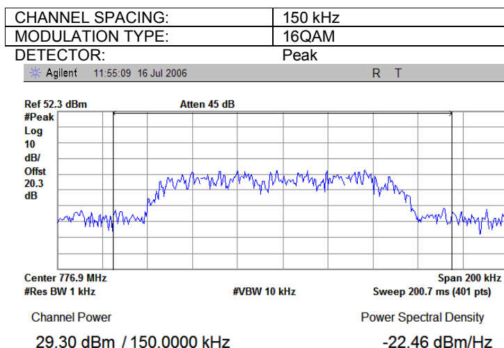
Plot 7.1.12 Peak output power test results at high frequency
