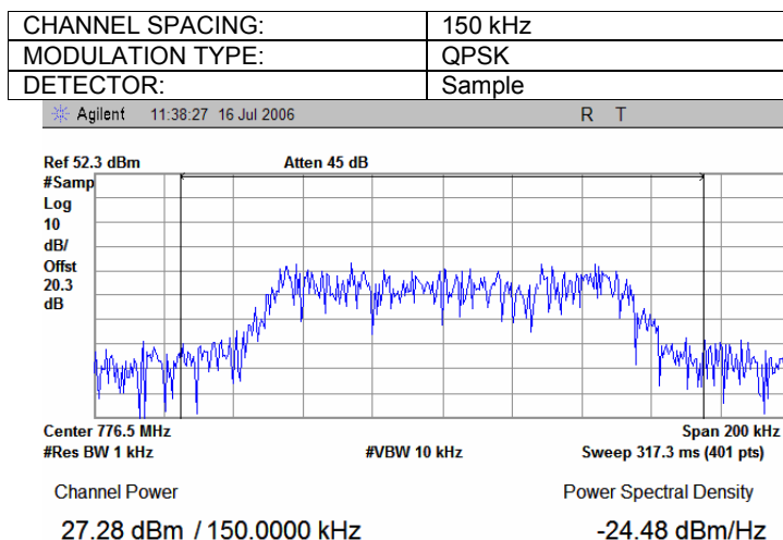
Plot 7.1.3 Average output power test results at mid frequency
