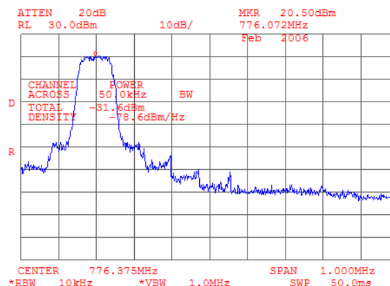
Plot 7.4.6 Adjacent channel coupled power measurements, low carrier frequency, QPSK
