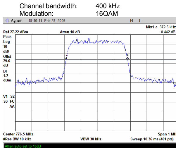
Plot 7.7.12 Occupied bandwidth test results at mid frequency
