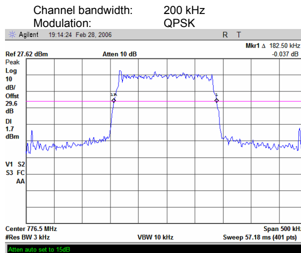
Plot 7.7.8 Occupied bandwidth test results at mid frequency
