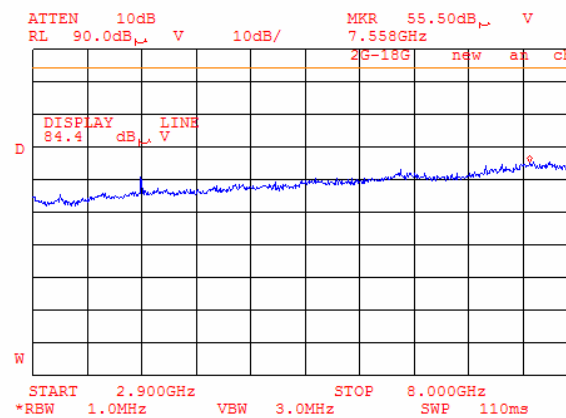
Plot 7.5.30 Radiated emission measurements in 2.9 – 8.0 GHz range
