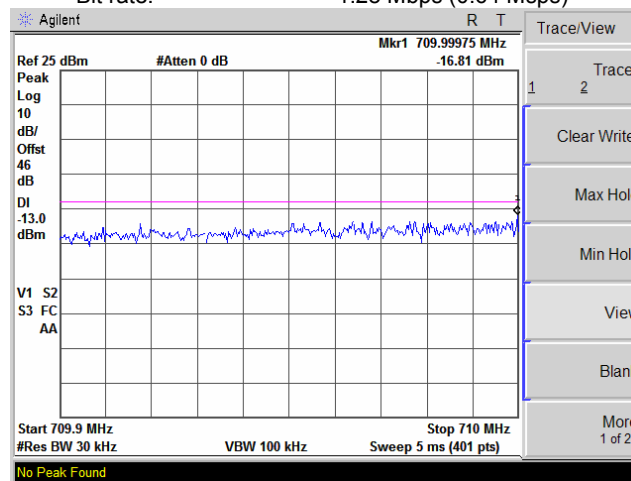
Plot 7.3.16 Spurious emissions at RF antenna connector, high channel band edge measurements
