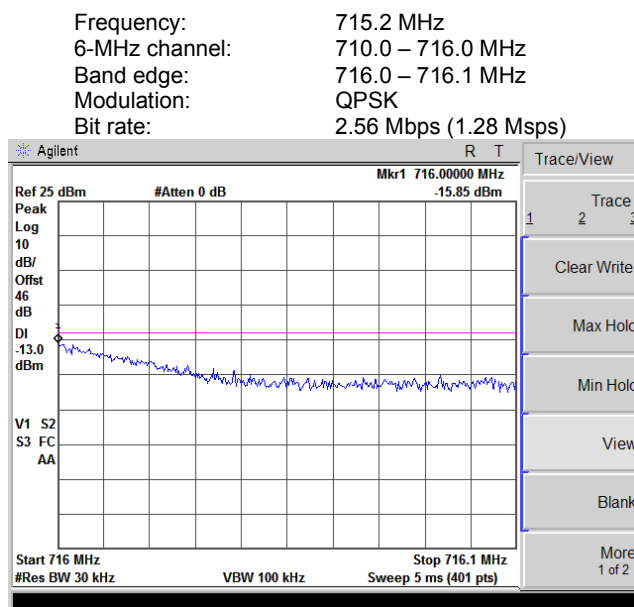
Plot 7.3.20 Spurious emissions at RF antenna connector, high channel band edge measurements
