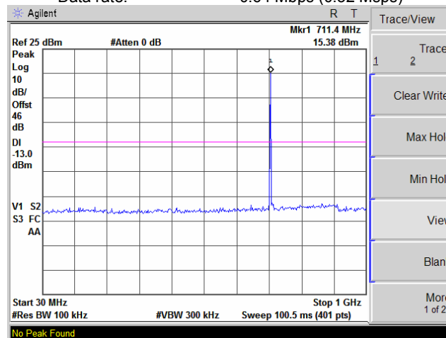
Plot 7.3.6 Spurious emission measurements at RF antenna connector, high channel
