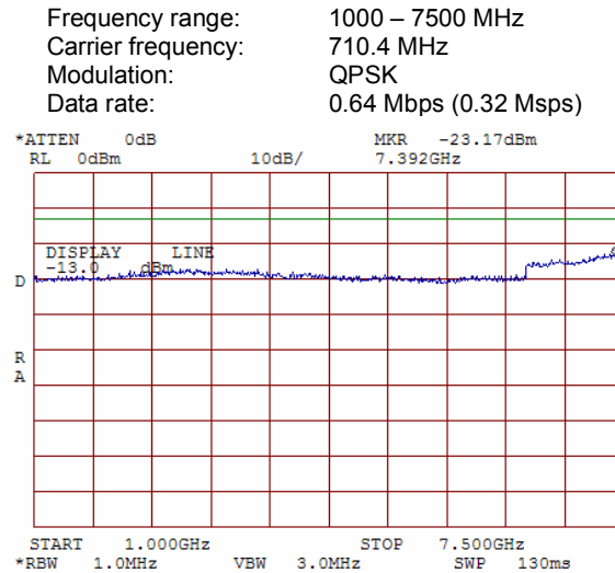
Plot 7.3.7 Spurious emission measurements at RF antenna connector, low channel
