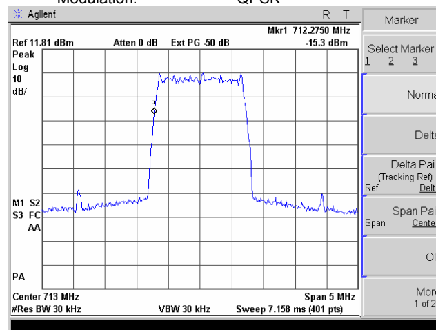
Plot 7.6.12 Occupied bandwidth test results at mid frequency
