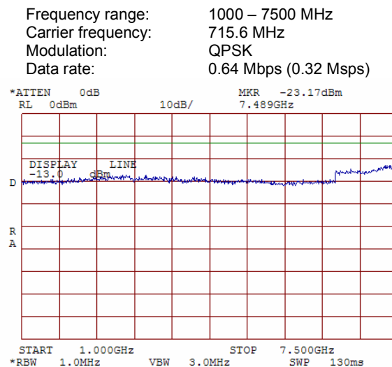
Plot 7.3.8 Spurious emission measurements at RF antenna connector, high channel
