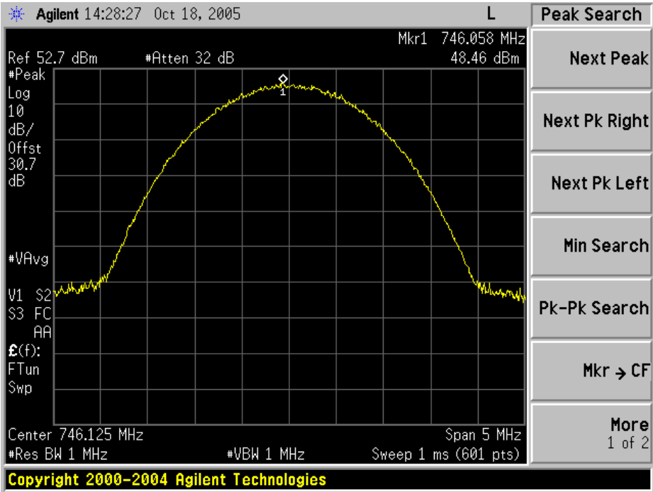
Plot#2 - QPSK AVERAGE Power Low Channel
