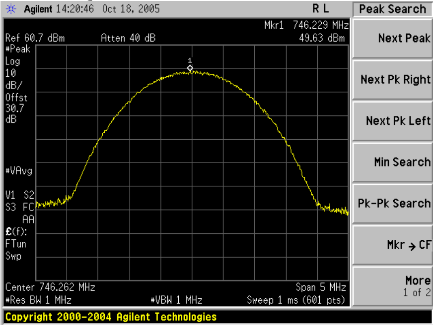
Plot # 5 - 16QAM PEAK Power Low Channel
