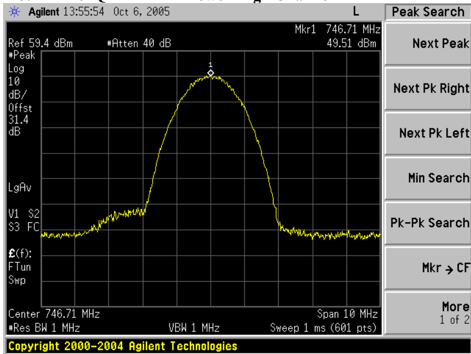
Plot # 11 - 64QAM PEAK Power High Channel
