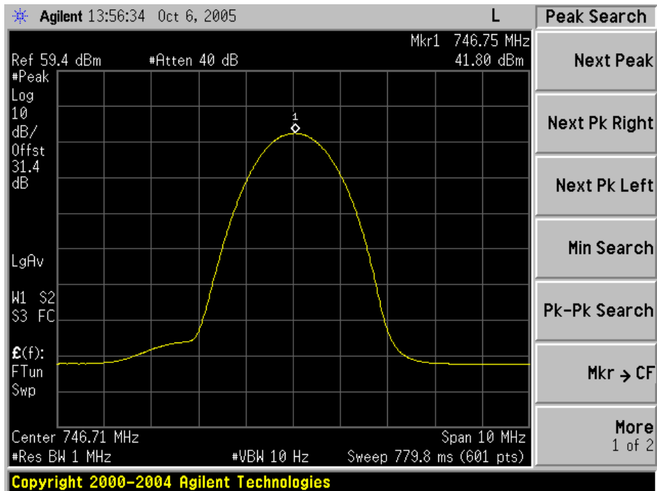
Plot # 12 - 64QAM AVERAGE Power High Channel
