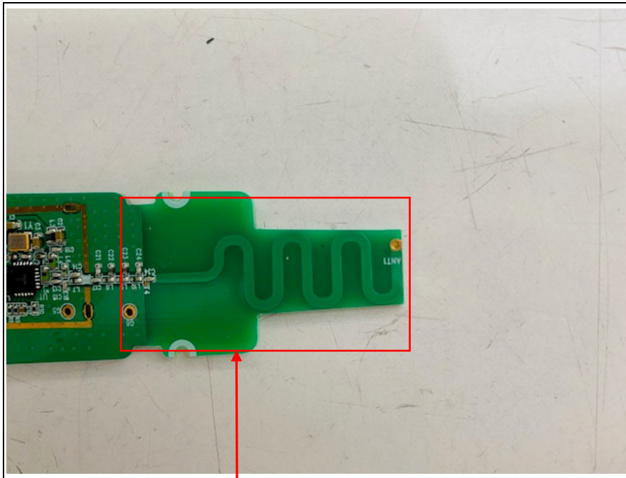
Pattern Antenna
