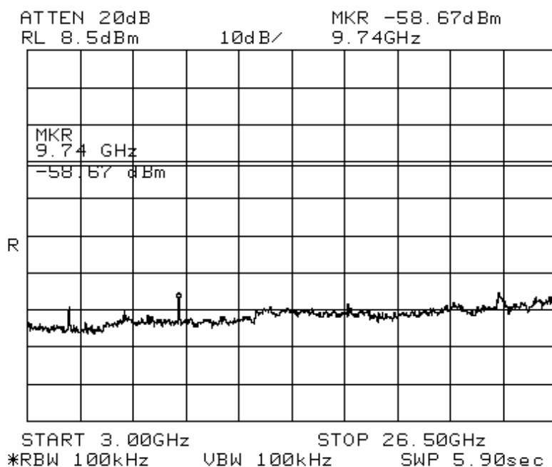
Middle Channel
