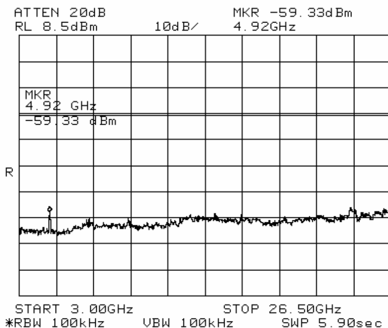
High Channel
