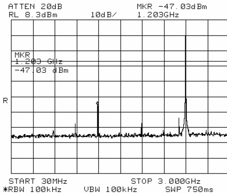
Low Channel
