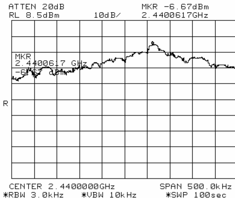
Middle Channel
