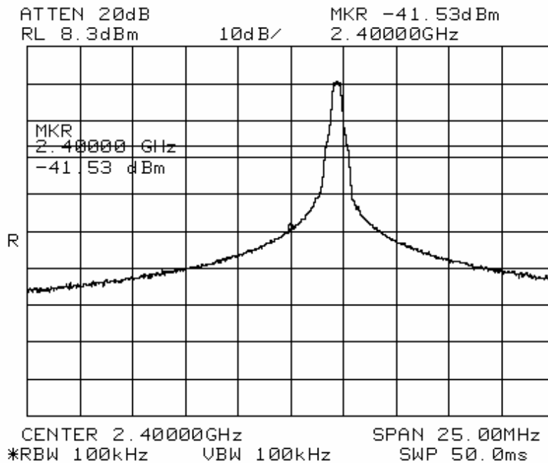
Low Channel
