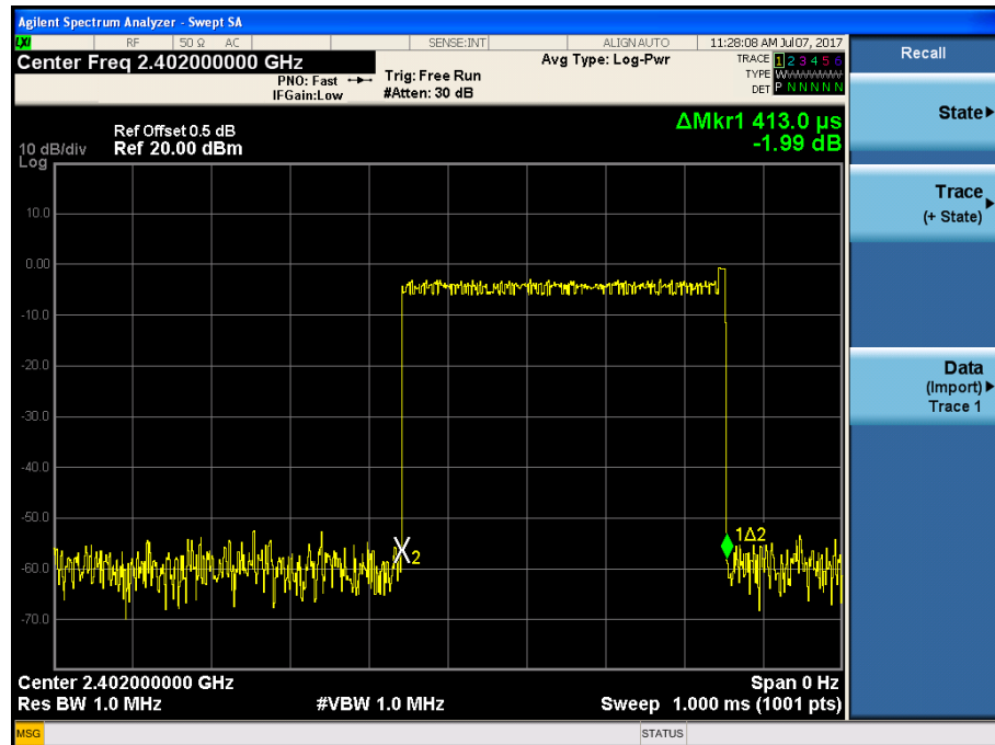
(Plot 4.8.2.A: Channel 00: 2402MHz @ 8DPSK @ DH1)
