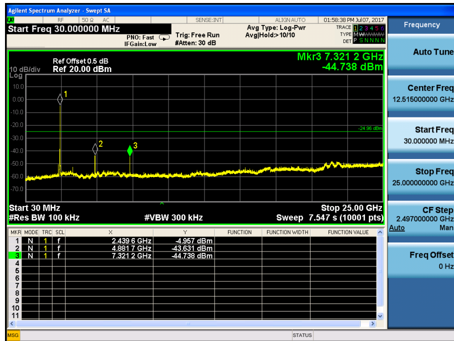
(Plot 4.9.2 B: Channel 39: 2441MHz @ @ 8DPSK)
