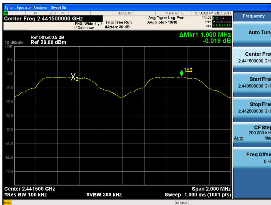
(Plot 4.6.1 A: Channel 39: 2441MHz @ GFSK)
