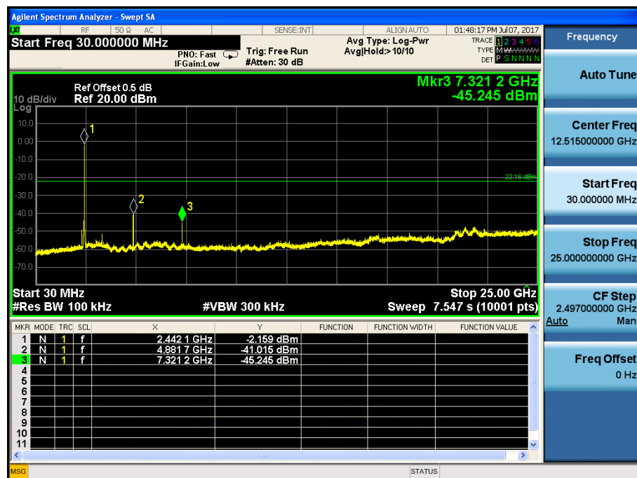
(Plot 4.9.1 B: Channel 39: 2441MHz @ GFSK)
