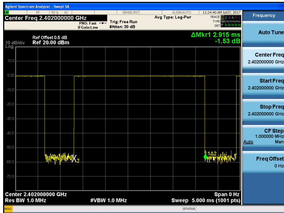
(Plot 4.8.1.C: Channel 00: 2402MHz @ GFSK @ DH5)
