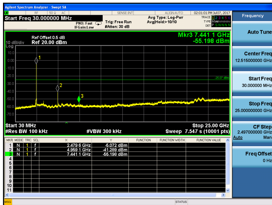
(Plot 4.9.2 C: Channel 78: 2480MHz @ @ 8DPSK)
