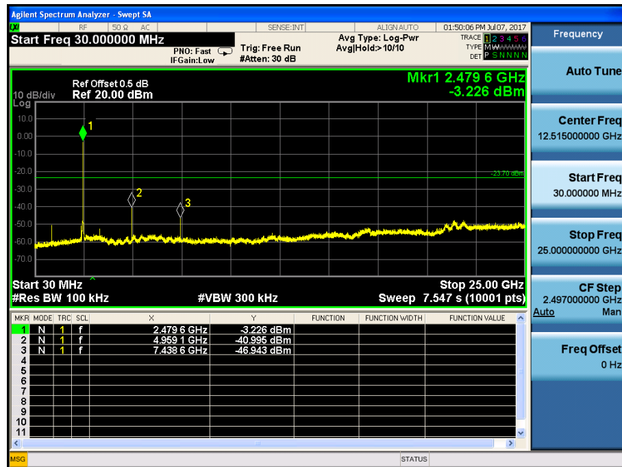
(Plot 4.9.1 C: Channel 78: 2480MHz @ GFSK)
