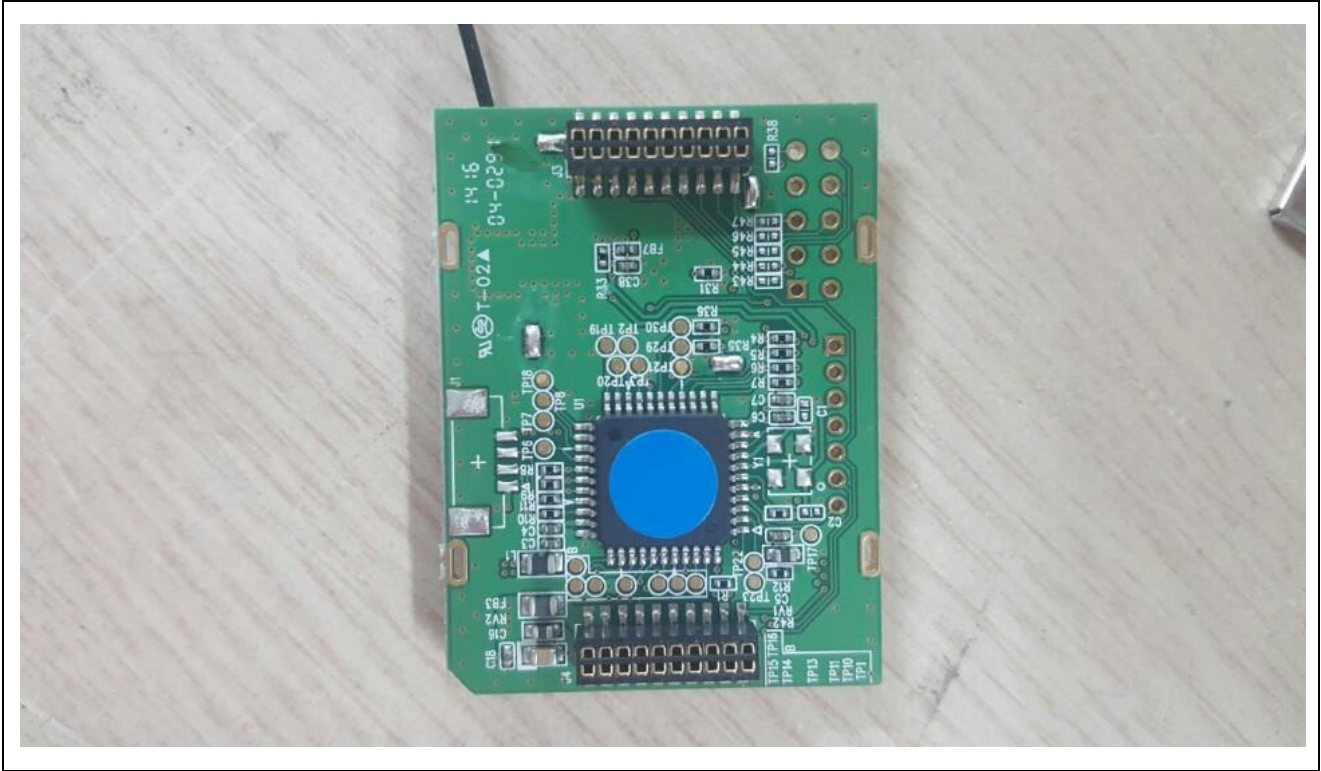
MainBoard-Rear
