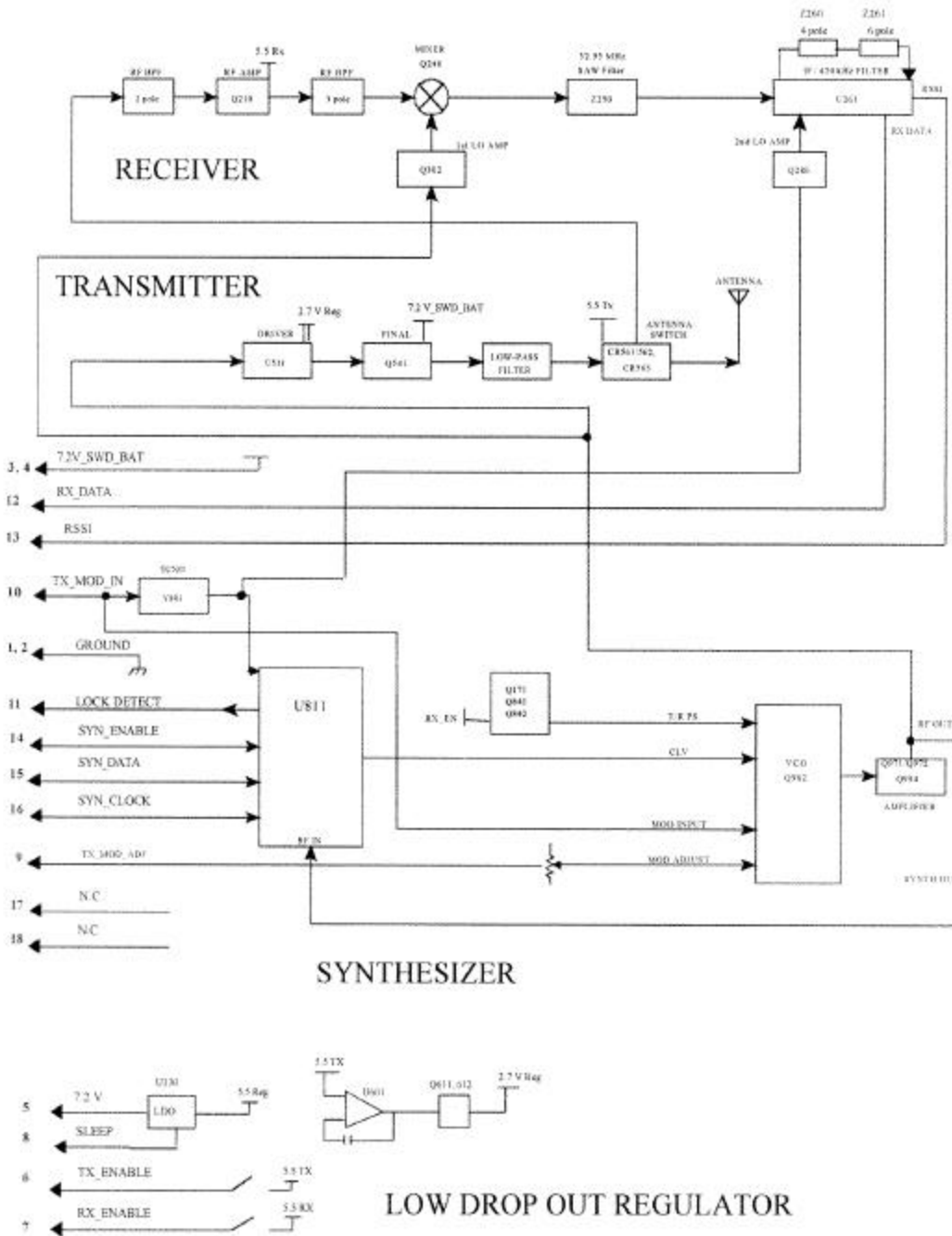
Figure 4-1 DATA TRANSCEIVER BLOCK DIAGRAM
