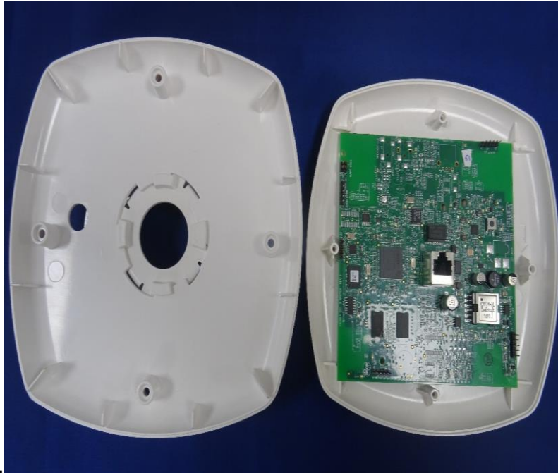
Photo 1:EUT with the outer enclosure removed
