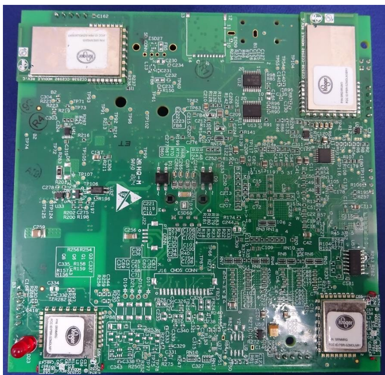
Photo 4: Rear view of internal PCB
