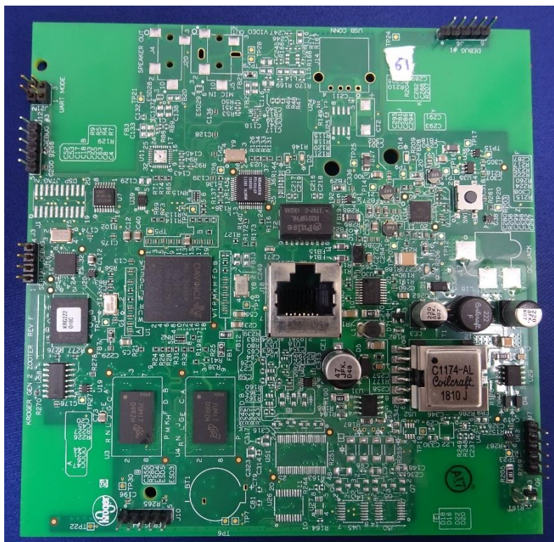
Photo 3:Top view of internal PCB
