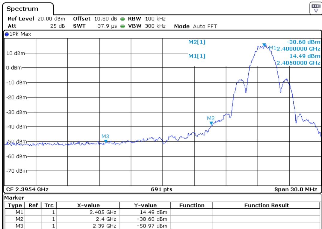
Channel low – 2405 MHz
