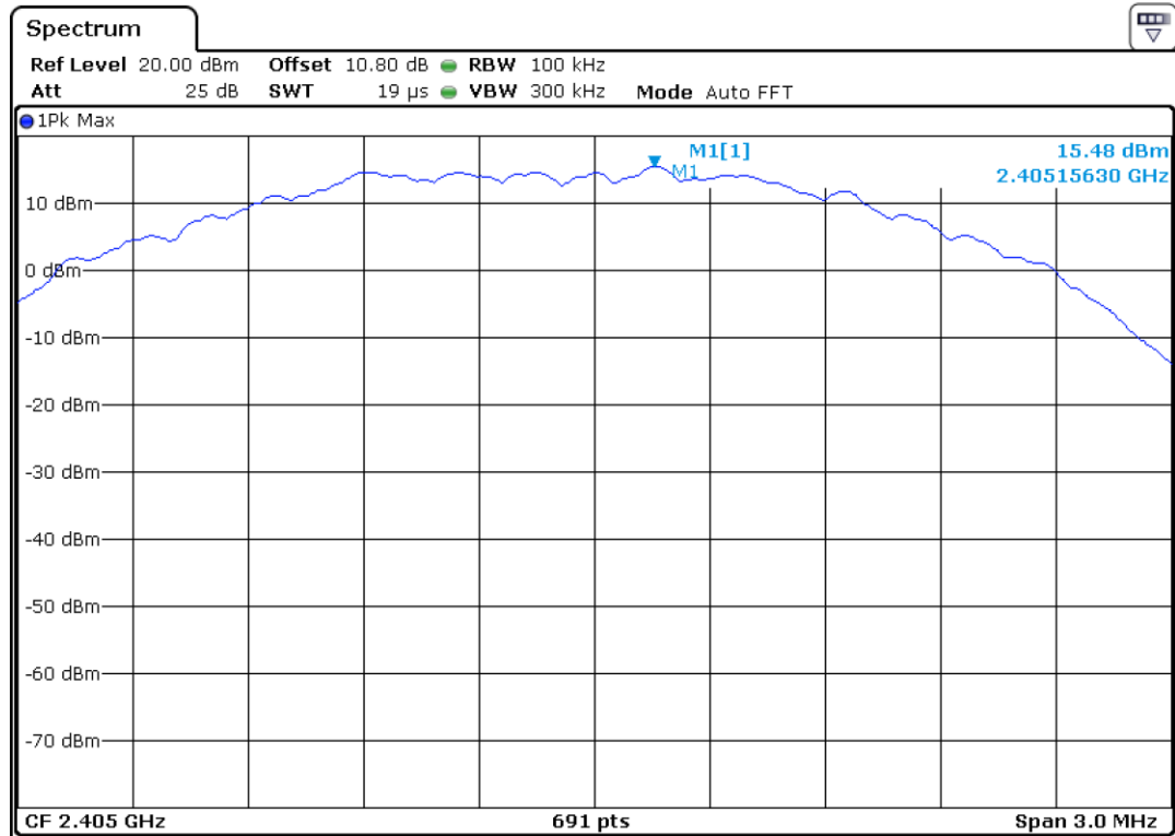
Reference Level Plot - Channel low 2405 MHz
