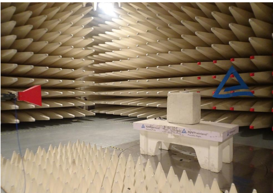
Photo 8: Horn antenna with horizontal polarization
