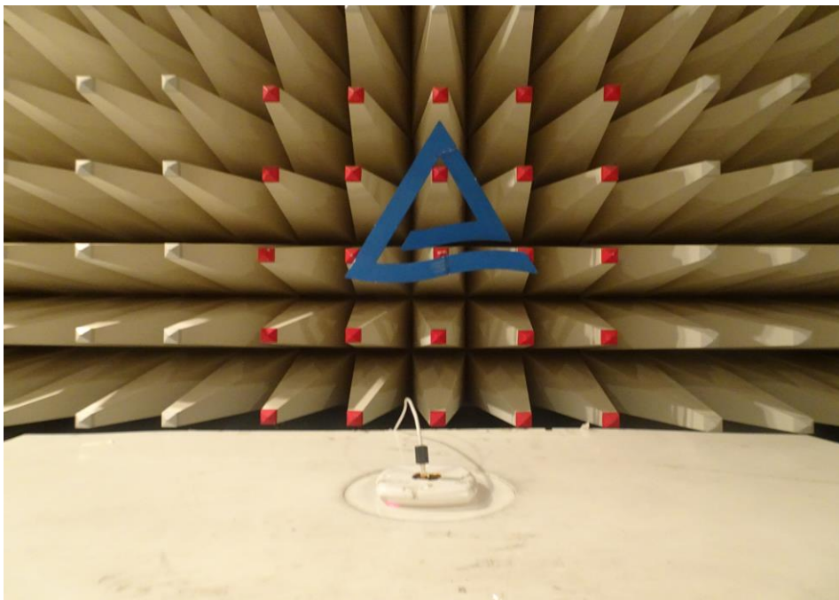
Photo 12: EUT setup
