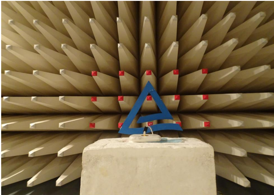
Photo 11: EUT setup
