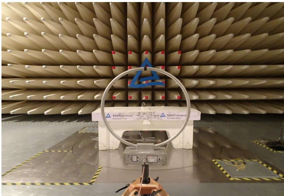
Photo 1 : Loop antenna with Parallel polarization
