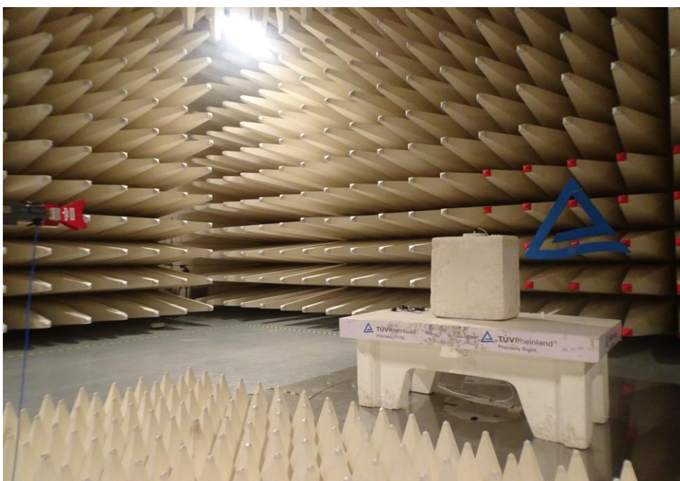
Photo 10: Horn antenna with horizontal polarization
