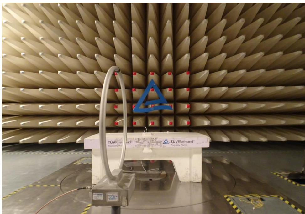
Photo 2: Loop antenna with Perpendicular polarization
