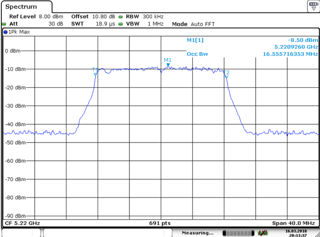
24 Mbps Channel mid – 5220 MHz OBW
