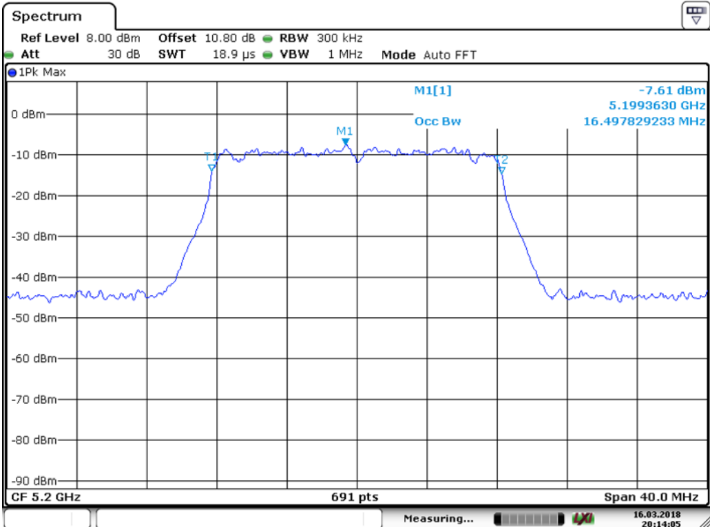
24 Mbps Channel mid – 5200 MHz OBW
