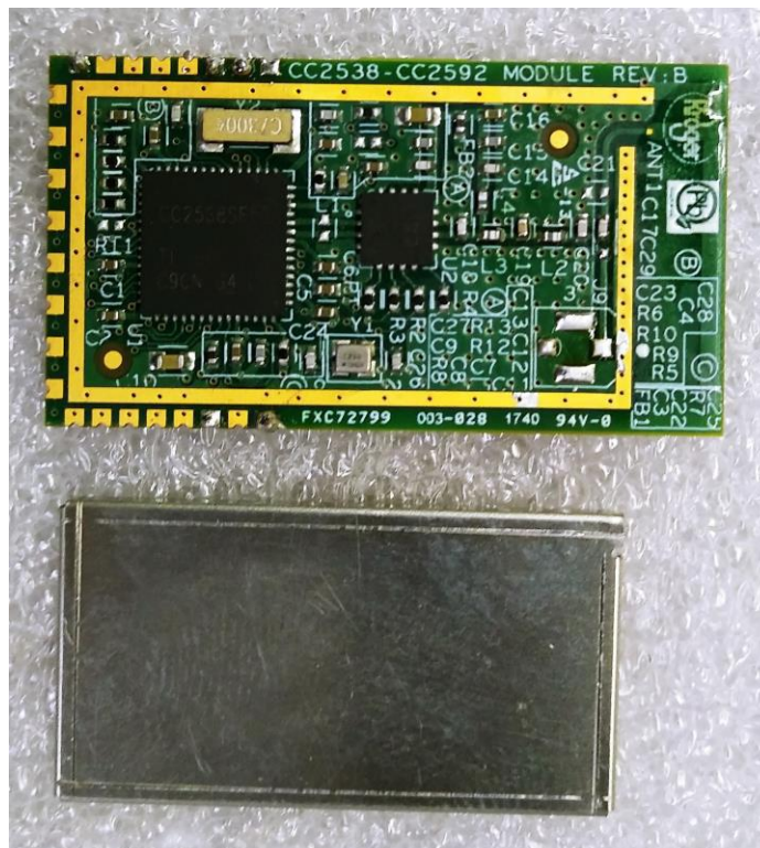
Photo 2: RF Module with shielding removed
