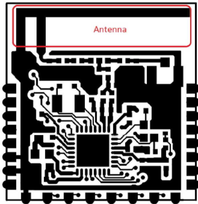
Photo 6: Antenna Trace Layout
