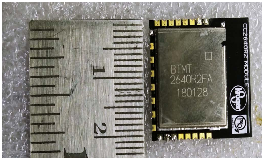
Photo 2: RF Module Dimensional View
