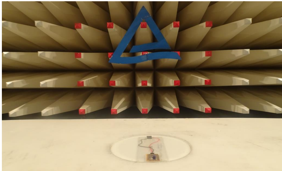
Photo 11: EUT setup
