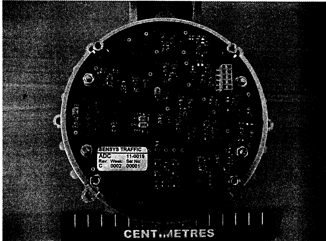
Internal view, PCB under antenna:
