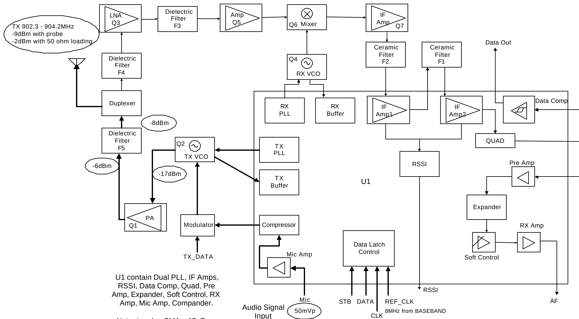
RF Signal Transmit Paths
