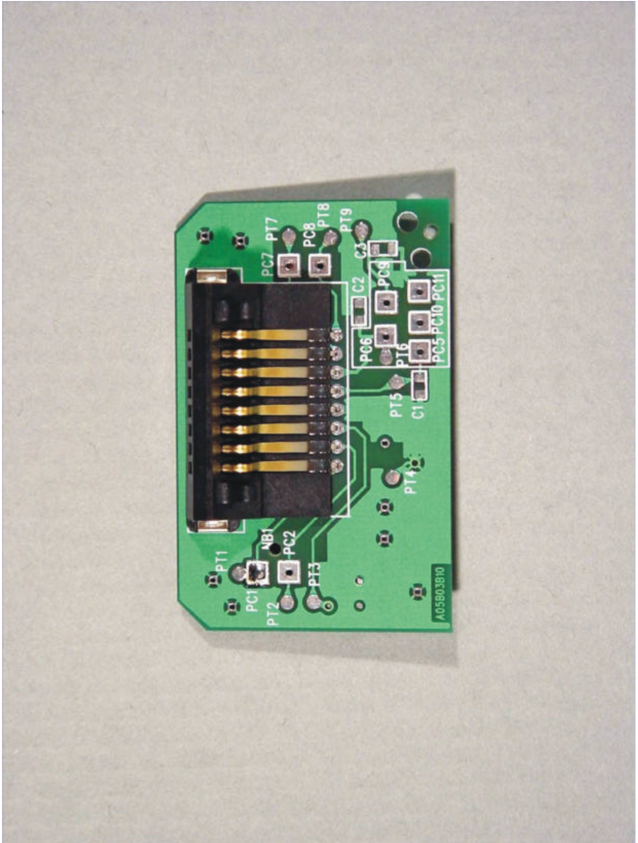
PC Interface PCBA Top View
