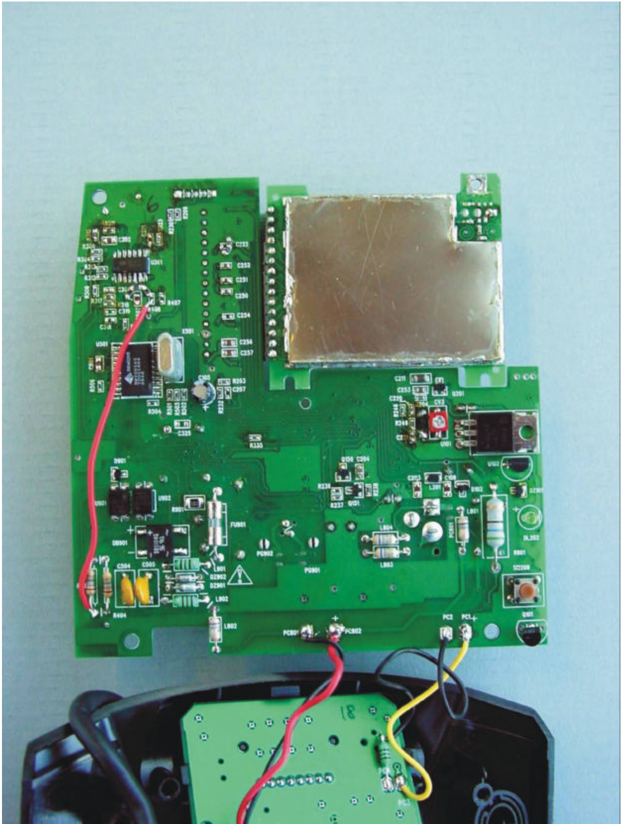
Base PCBA Top View
