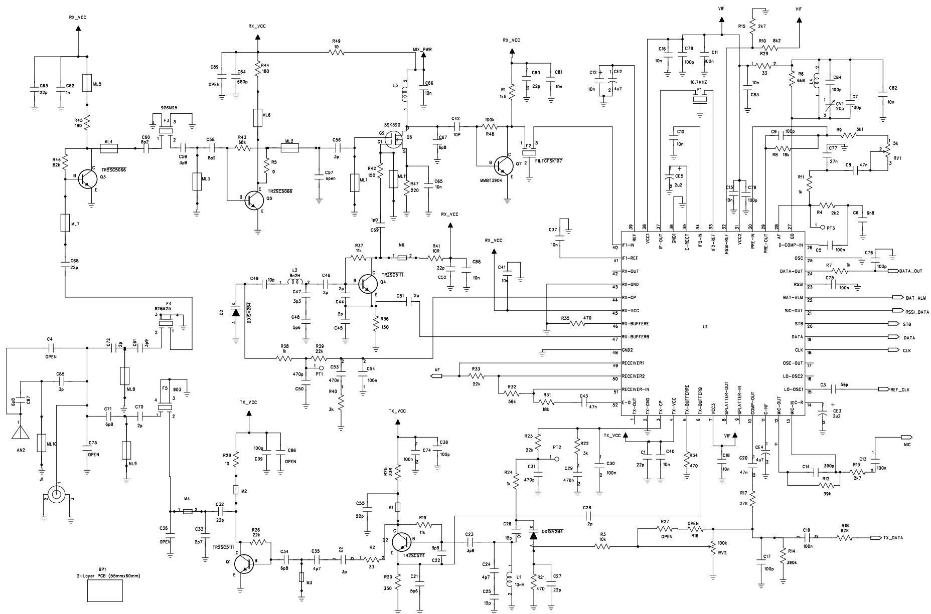
BASE UNIT RF SCHEMATIC DIAGRAM
