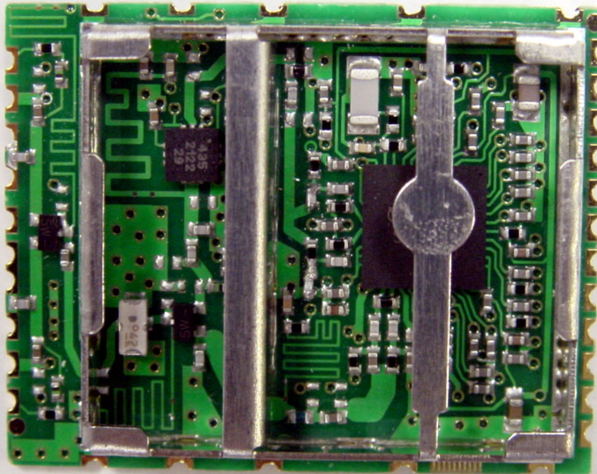
BASE RF PCBA
